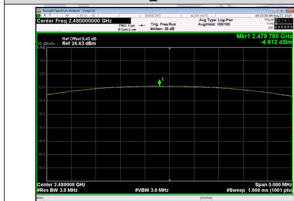
Peak Output Power GFSK_Channel 78
