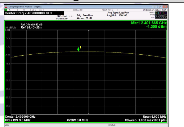
Peak Output Power \pi/4 DQPSK_Channel 0
