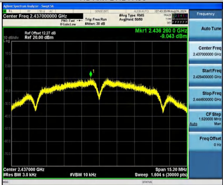
11B-Ant1-2437-PASS
