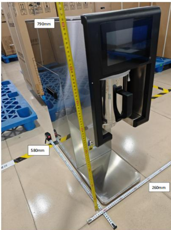
6. HZ-6ZCF-33SWG-JP Size information is as follows: 260mm*580mm*790mm
