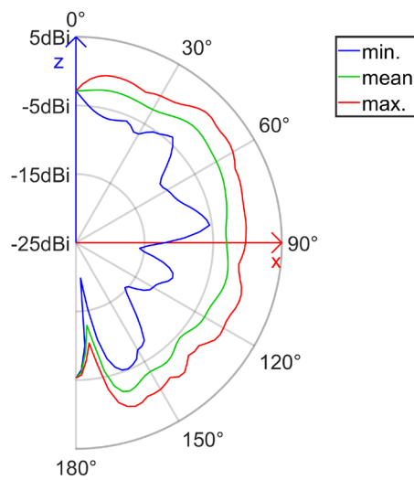
radiation pattern of the antenna (elevation cut) realized gain (E_Total, Freq = 4400.00 MHz)
