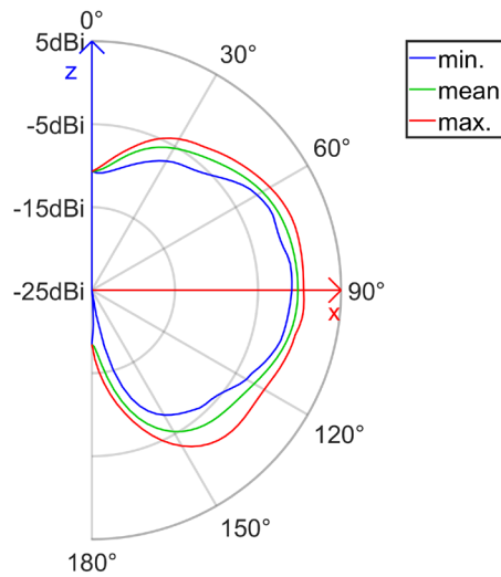
radiation pattern of the antenna (elevation cut) realized gain (E_Total, Freq = 1510.90 MHz)
