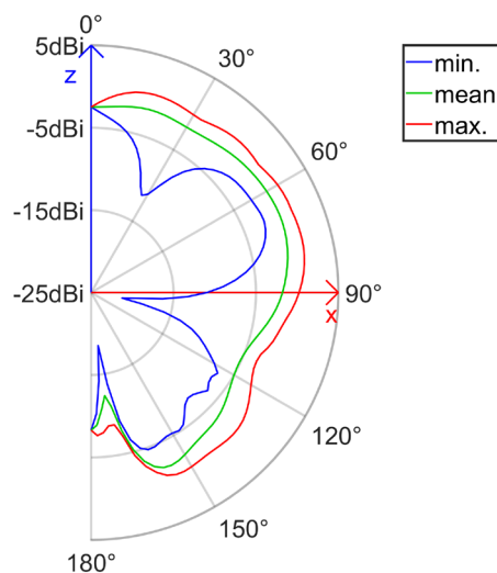
radiation pattern of the antenna (elevation cut) realized gain (E_Total, Freq = 2690.00 MHz)
