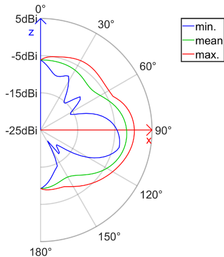
radiation pattern of the antenna (elevation cut) realized gain (E_Total, Freq = 698.00 MHz)
