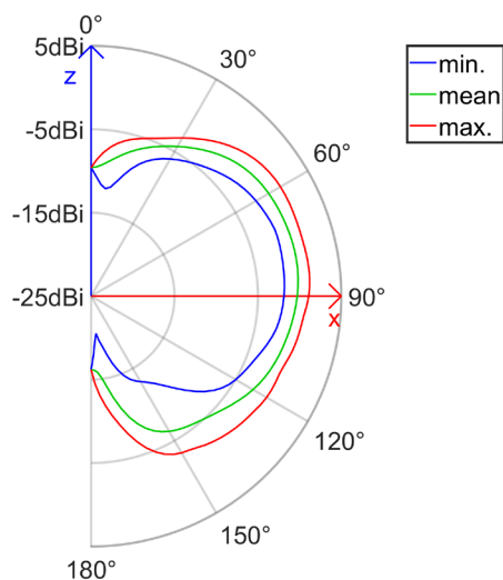
radiation pattern of the antenna (elevation cut) realized gain (E_Total, Freq = 1710.00 MHz)
