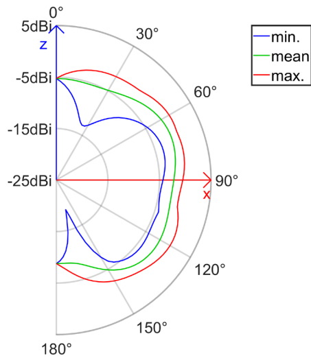
radiation pattern of the antenna (elevation cut) realized gain (E_Total, Freq = 1475.90 MHz)
