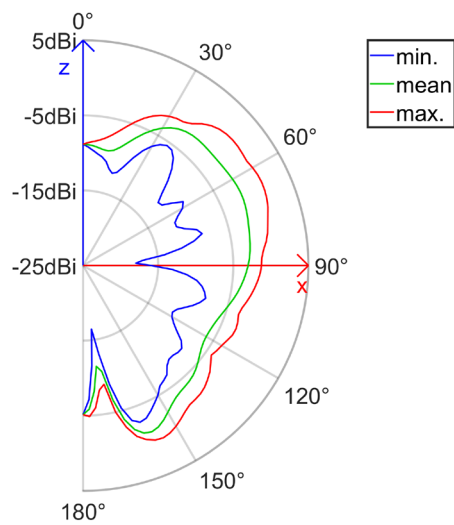
radiation pattern of the antenna (elevation cut) realized gain (E_Total, Freq = 4200.00 MHz)
