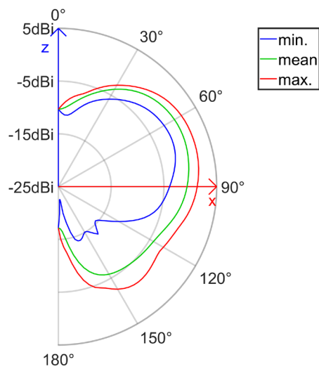
radiation pattern of the antenna (elevation cut) realized gain (E_Total, Freq = 2170.00 MHz)
