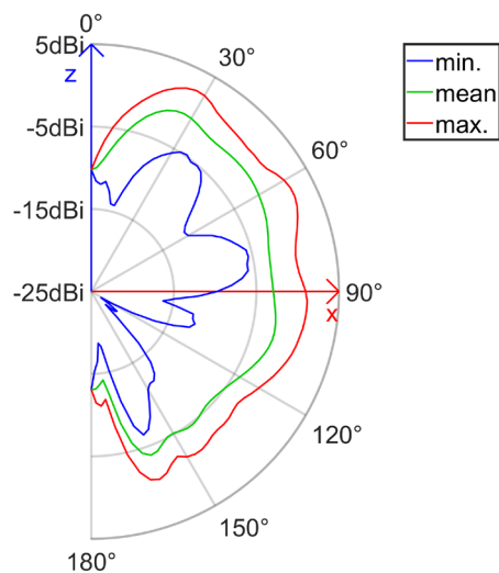
radiation pattern of the antenna (elevation cut) realized gain (E_Total, Freq = 4700.00 MHz)
