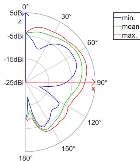
radiation pattern of the antenna (elevation cut) realized gain (E_Total, Freq = 2500.00 MHz)
