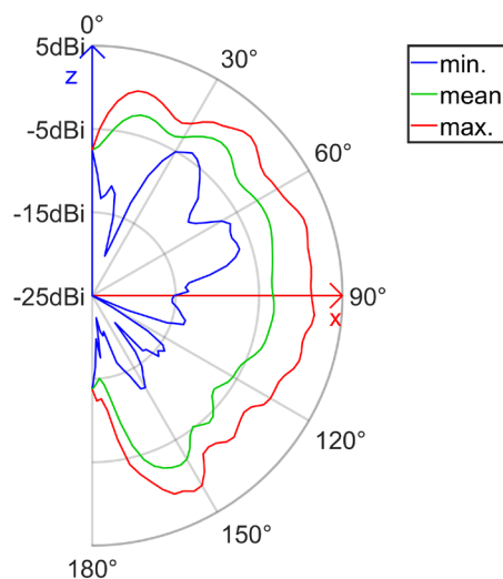
radiation pattern of the antenna (elevation cut) realized gain (E_Total, Freq = 4990.00 MHz)
