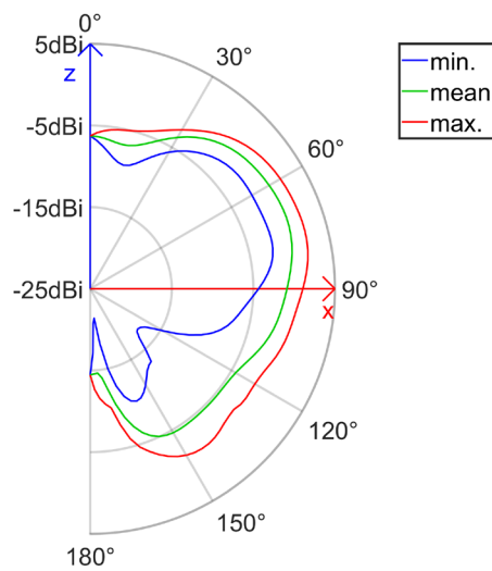
radiation pattern of the antenna (elevation cut) realized gain (E_Total, Freq = 2300.00 MHz)
