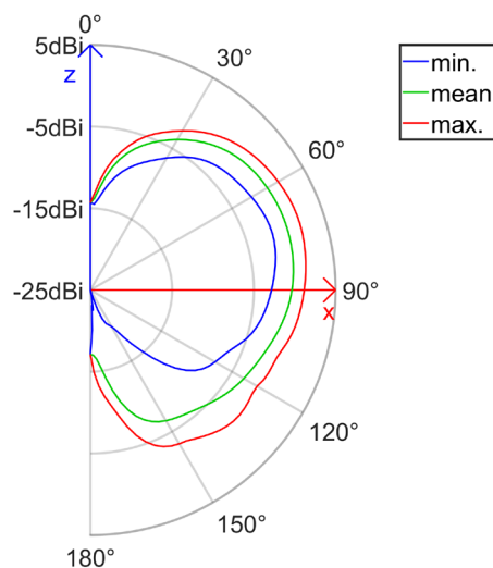
radiation pattern of the antenna (elevation cut) realized gain (E_Total, Freq = 1850.00 MHz)
