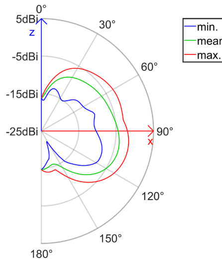
radiation pattern of the antenna (elevation cut) realized gain (E_Total, Freq = 830.00 MHz)
