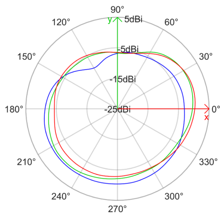
radiation pattern of the antenna realized partial average gain (E_Total, Theta = [60.00 - 90.00]°)
