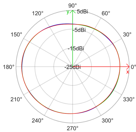
radiation pattern of the antenna realized partial average gain (E_Total, Theta = [60.00 - 90.00]°)
