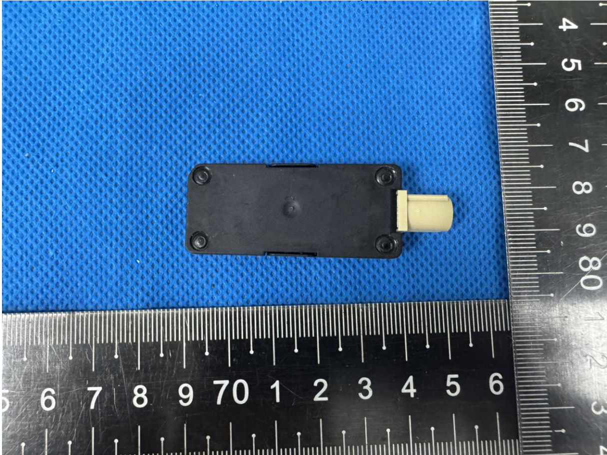
Photo16 External Antenna (4N0.035.500)
