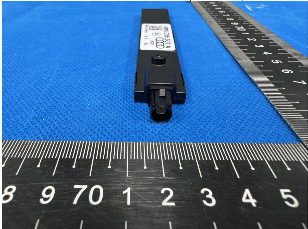
Photo14 DRX External Antenna 2(4M0.035.504.A)
