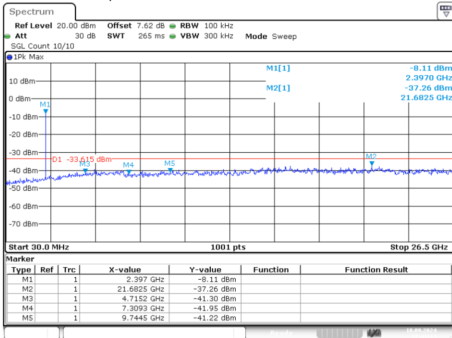
Tx. Spurious NVNT GFSK 2405MHz Ant1 Emission
