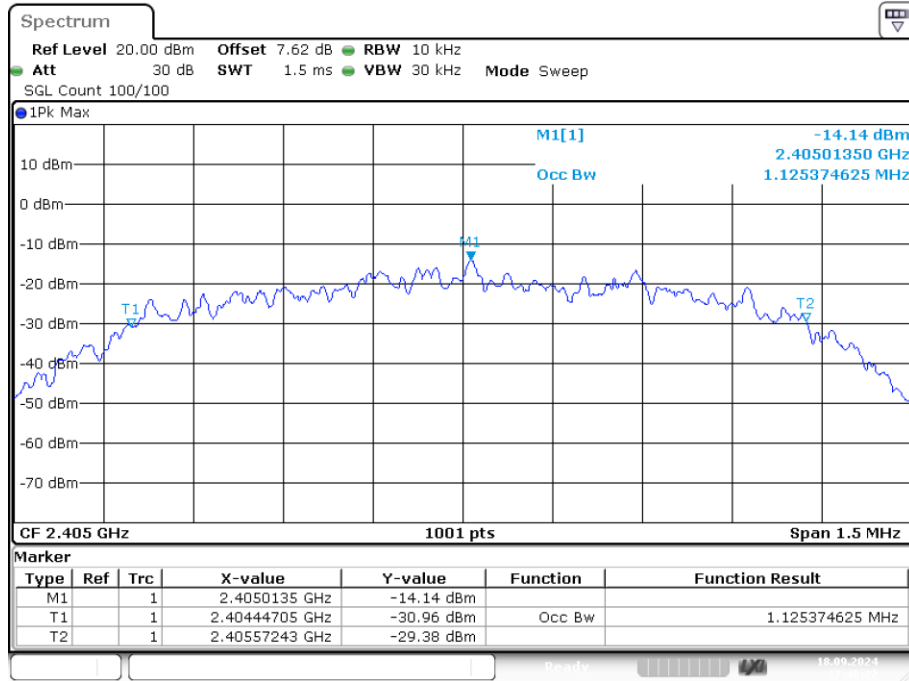
OBW NVNT GFSK 2405MHz Ant1
