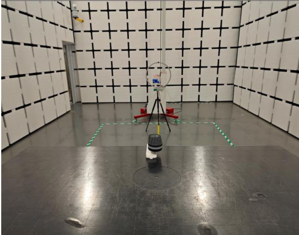
Spurious Radiation Emissions Test (<30M)
