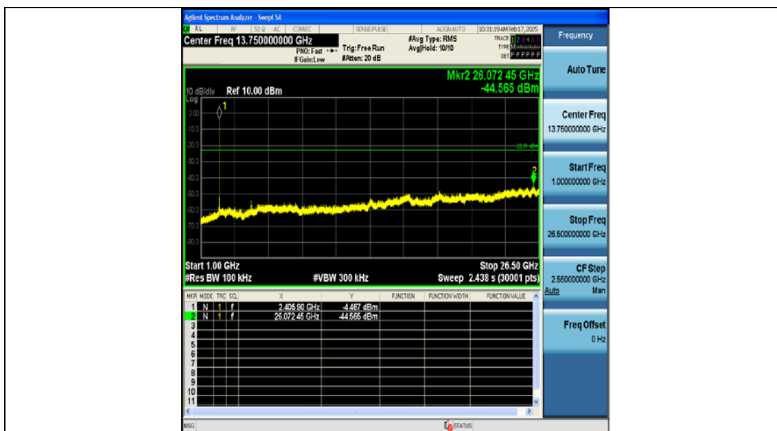
SRD-Ant1-2405-1000~26500-PASS
