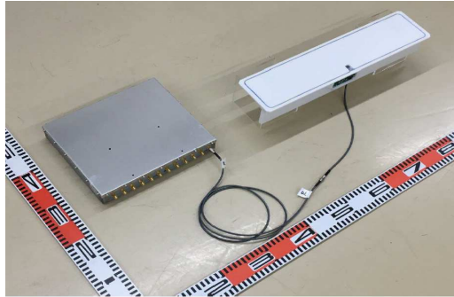
Dealer Antenna
