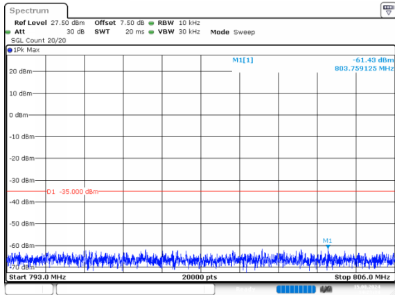
5MHz_Low_QPSK_1@0(793MHz~806MHz)
