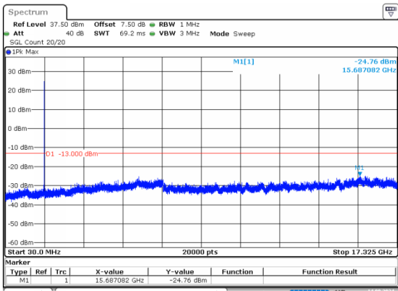
3MHz_Middle_QPSK_1@0
