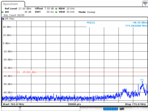
5MHz_Low_QPSK_1@0(763MHz~775MHz)
