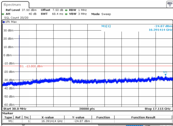
3MHz_Low_QPSK_1@0
