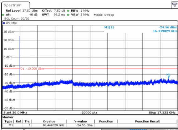
1.4MHz_Middle_QPSK_1@0
