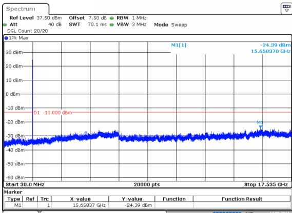
3MHz_High_QPSK_1@0
