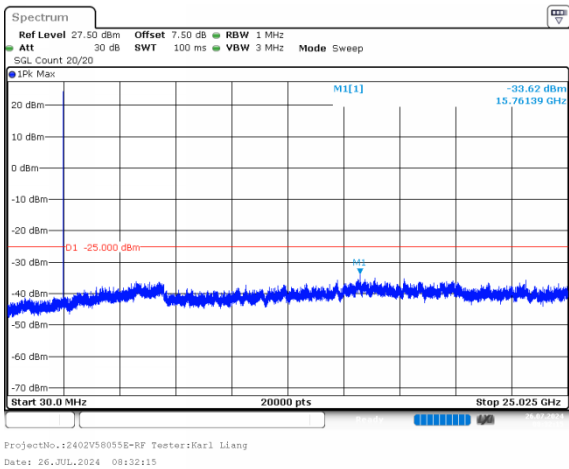
5MHz_High_QPSK_1@0
