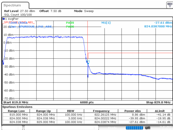
1_5MHz_High_QPSK_25@0
