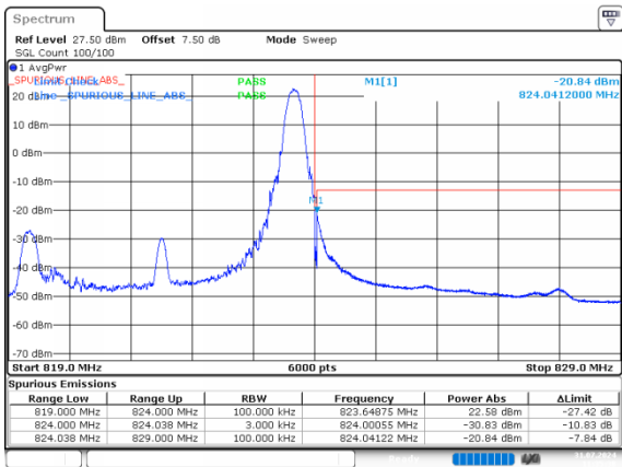
1_5MHz_High_QPSK_1@24
