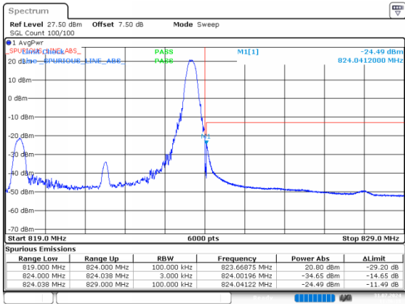
1_5MHz_High_16QAM_1@24
