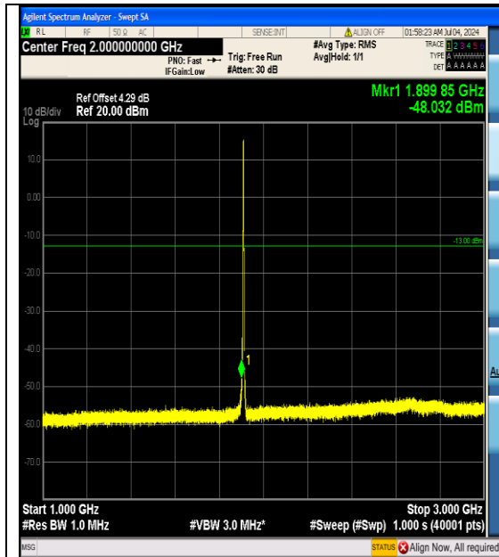
Band2_3MHz_16QAM_19185_15RB#0_1000~3000_1000~3000
