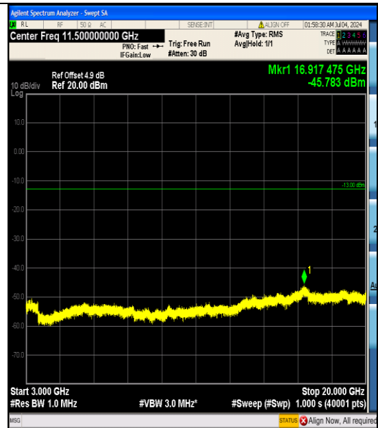
Band2_3MHz_16QAM_19185_15RB#0_3000~20000_0000_3000~20000
