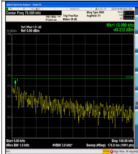
Band2_5MHz_QPSK_18625_25RB#0_0.009~0.15_0.009~0.15
