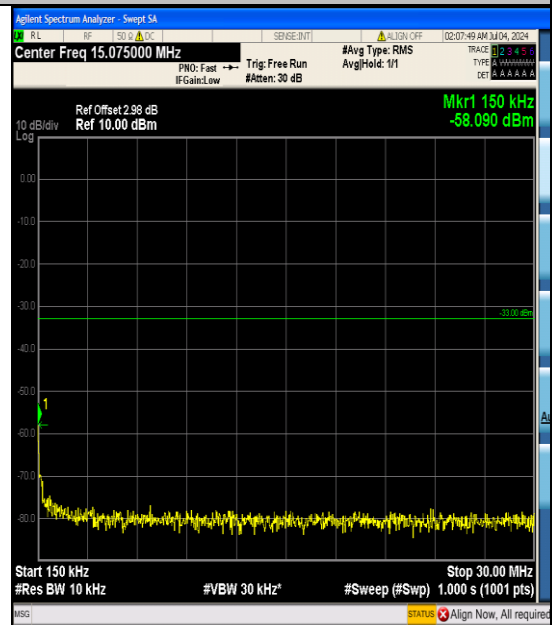
Band2_5MHz_QPSK_18625_25RB#0_0.15~30_0.15~30
