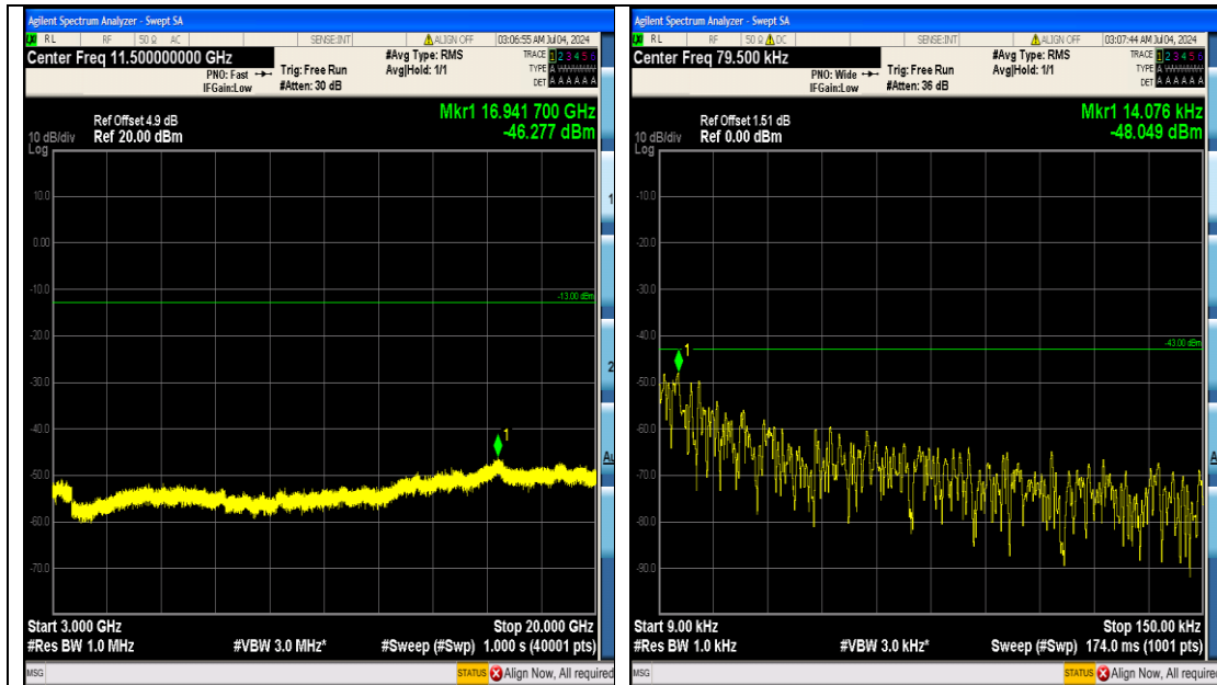
Band4_3MHz_16QAM_20175_15RB#0_3000~20000_3000~20000
