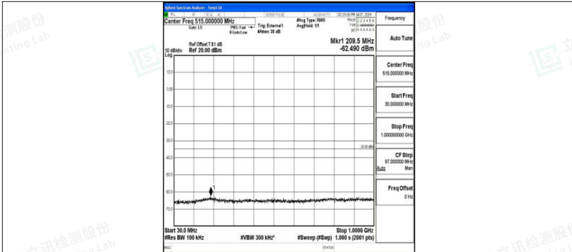
Band38_5MHz_16QAM_38225_1RB#0_30~1000_30~1000
