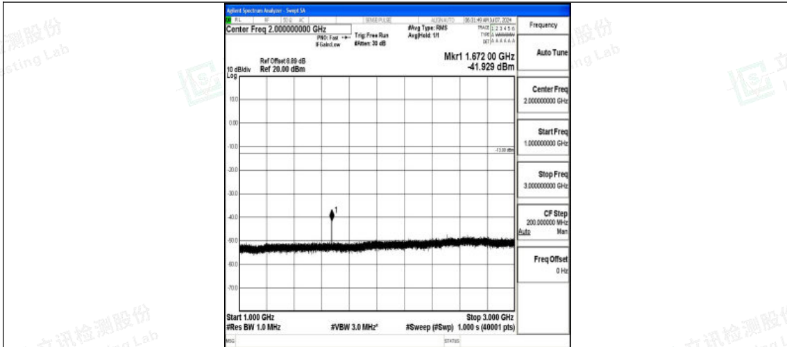
Band5_1.4MHz_16QAM_20525_1RB#0_1000~3000_1000~3000
