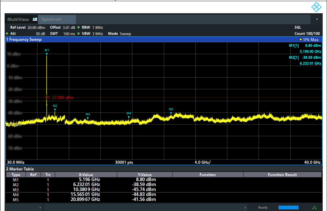
Tx. Spurious NVNT a 5200MHz Ant1 Emission
