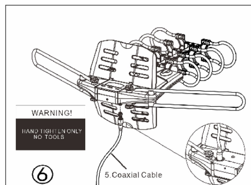
Step 6: Install the RG6 coaxial cable with waterproof cap on the F Connector of the main unit and put on the waterproof cap.
