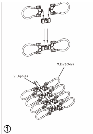
Step 1: Assemble 8pcs of directors
