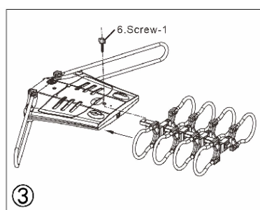
Step 3: Fix the directors by M4*18mm screw
