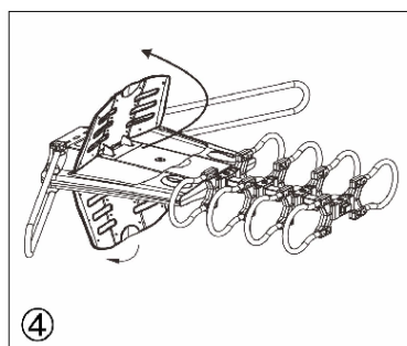
Step 4: Unfold the antenna reflectors.
