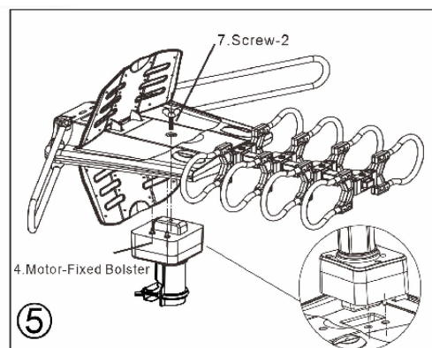
Step 5: Fix the motor bolster by M5*25mm bolt.
