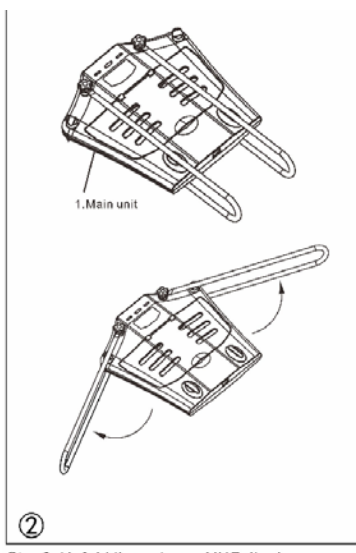
Step 2: Unfold the antenna VHF dipoles
