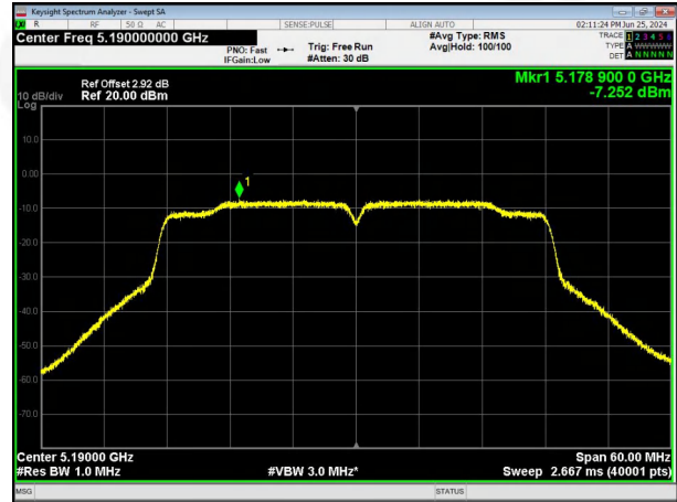
ANT2 (802.11n40) PSD plot on channel 38
