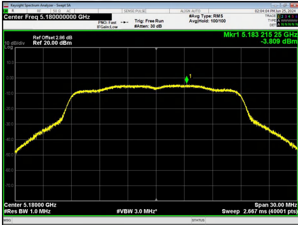
ANT2 (802.11n20) PSD plot on channel 36
