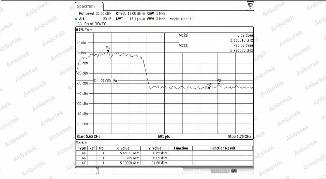
11N40SISO-Ant1-5670-PASS
