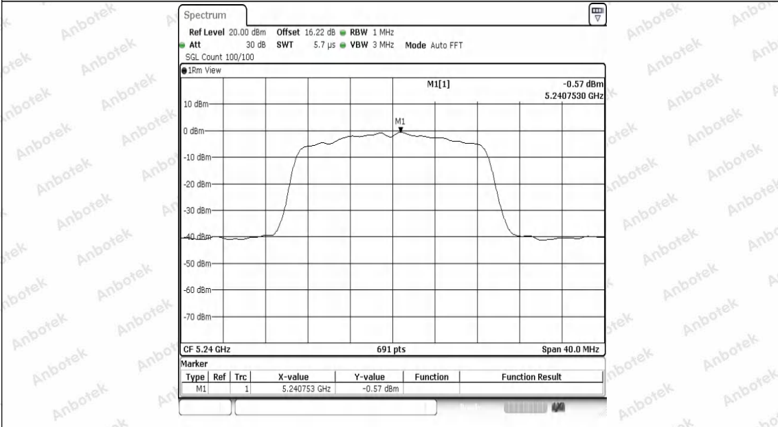
11AC20SISO-Ant1-5240-PASS
