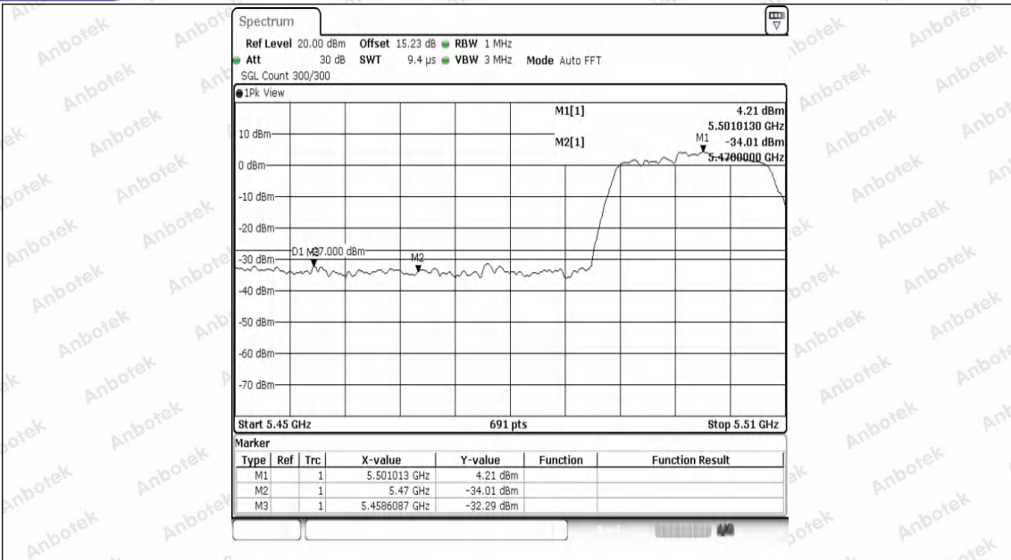
11AC20SISO-Ant1-5500-PASS
