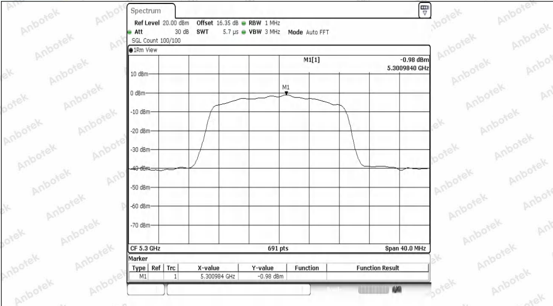
11N20SISO-Ant1-5300-PASS
