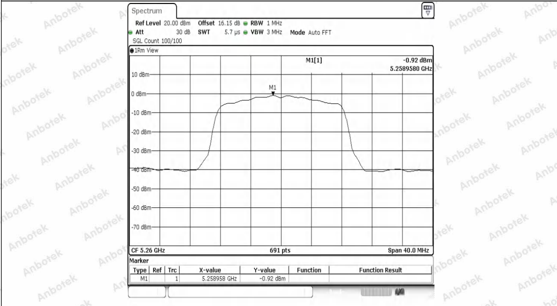
11A-Ant1-5260-PASS
