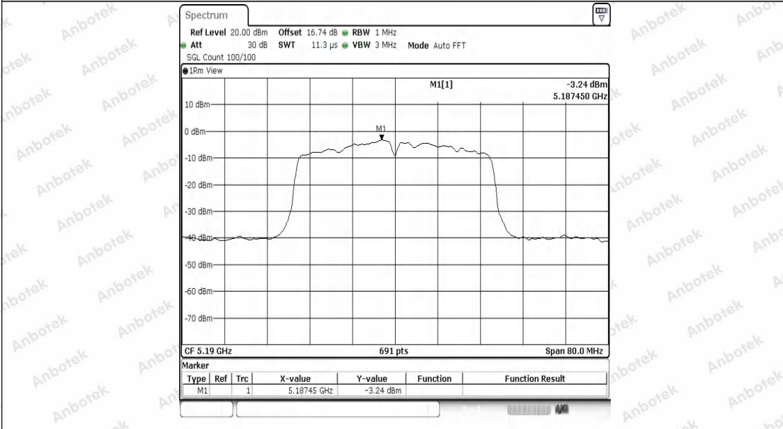
11AC40SISO-Ant1-5190-PASS
