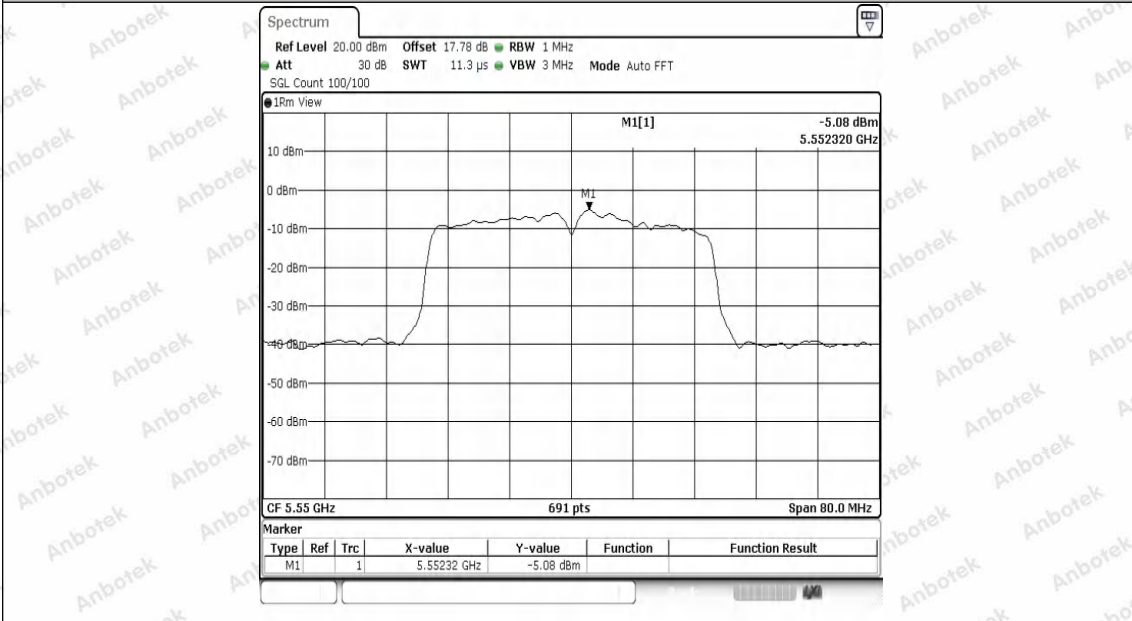
11N40SISO-Ant1-5550-PASS
