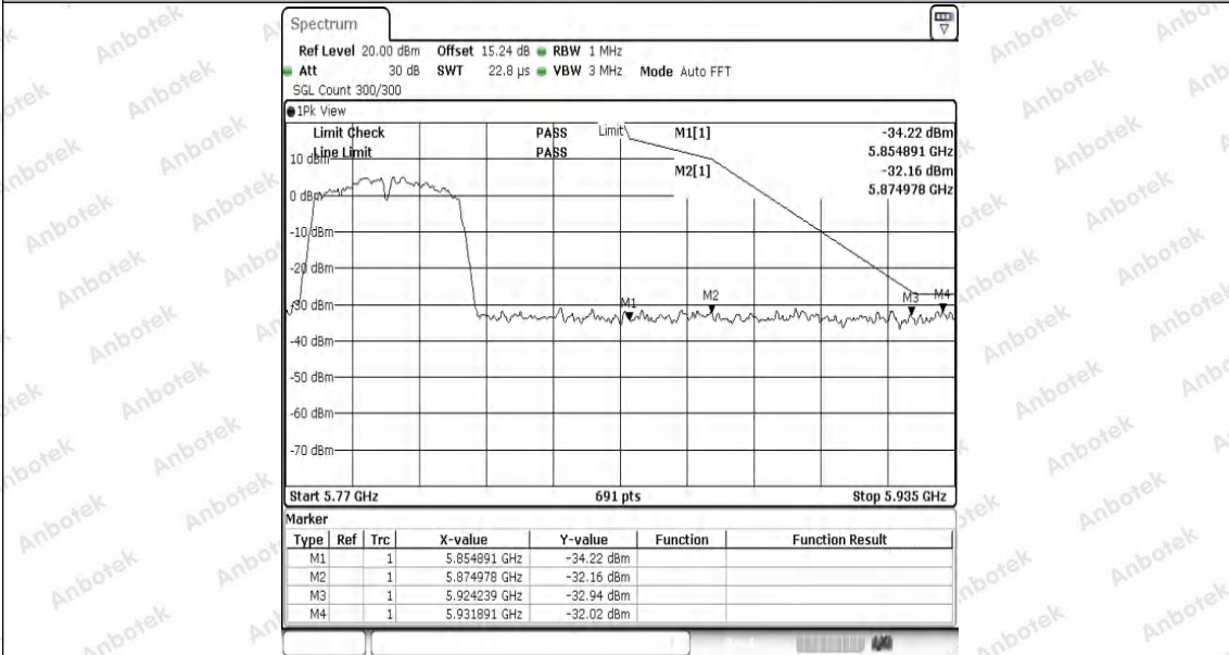
11AC40SISO-Ant1-5795-PASS
