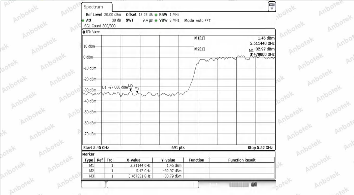
11N40SISO-Ant1-5510-PASS
