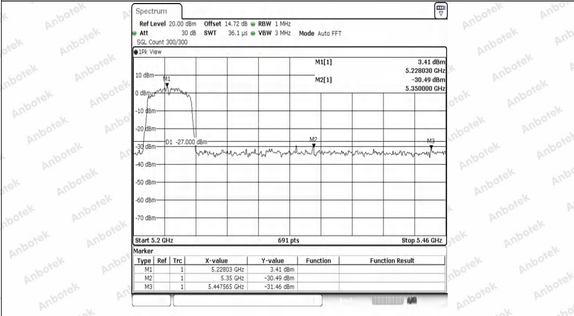
11AC40SISO-Ant1-5230-PASS
