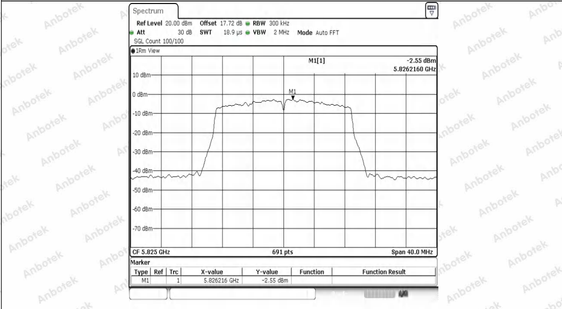
11N20SISO-Ant1-5825-PASS
