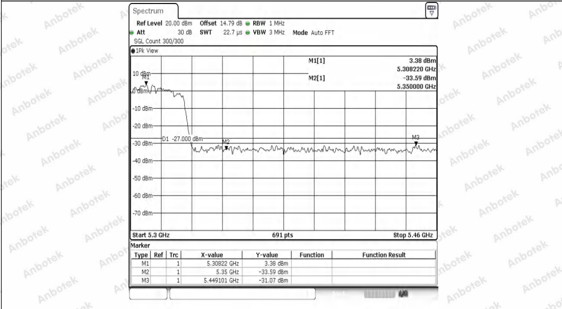
11AC40SISO-Ant1-5310-PASS
