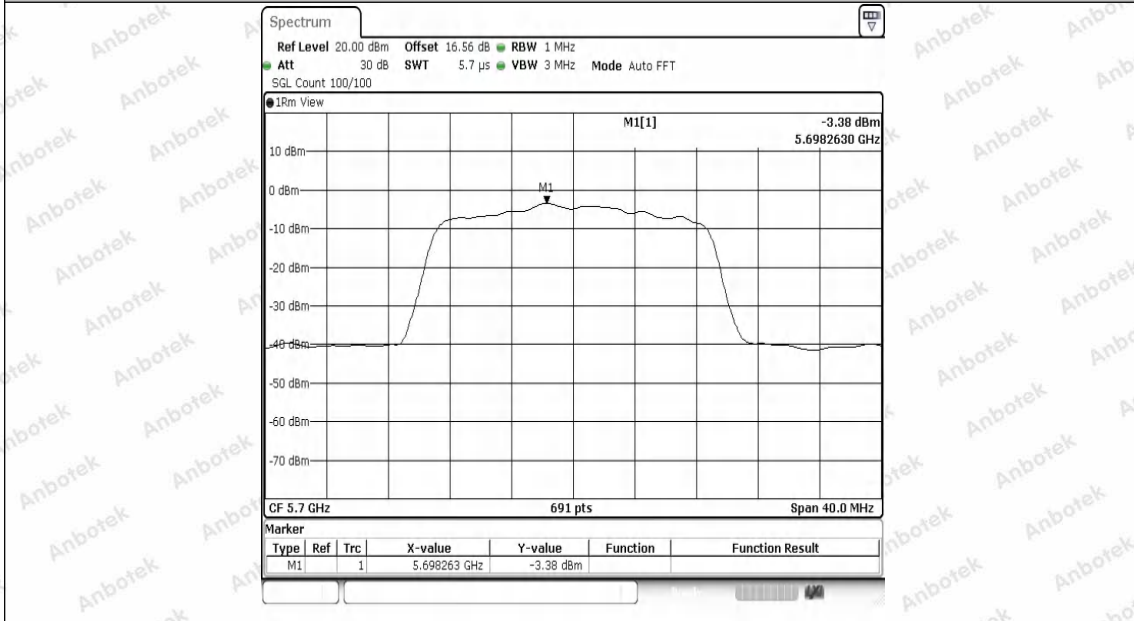
11AC20SISO-Ant1-5700-PASS
