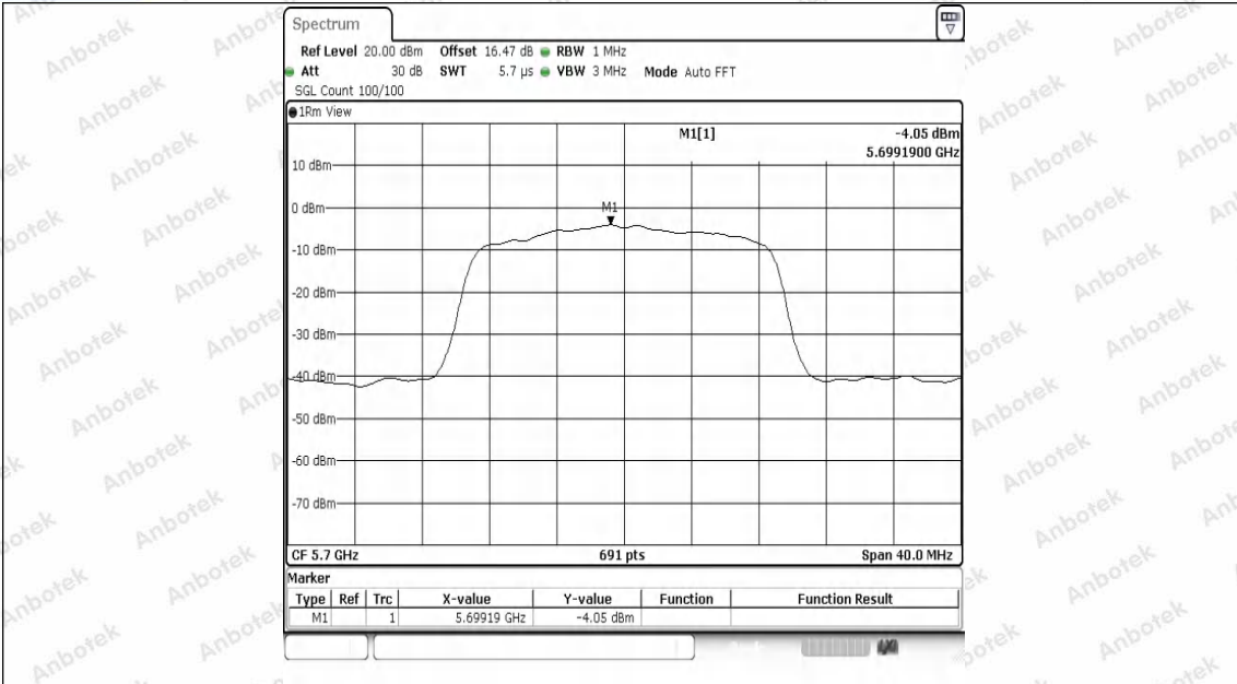
11N20SISO-Ant1-5700-PASS
