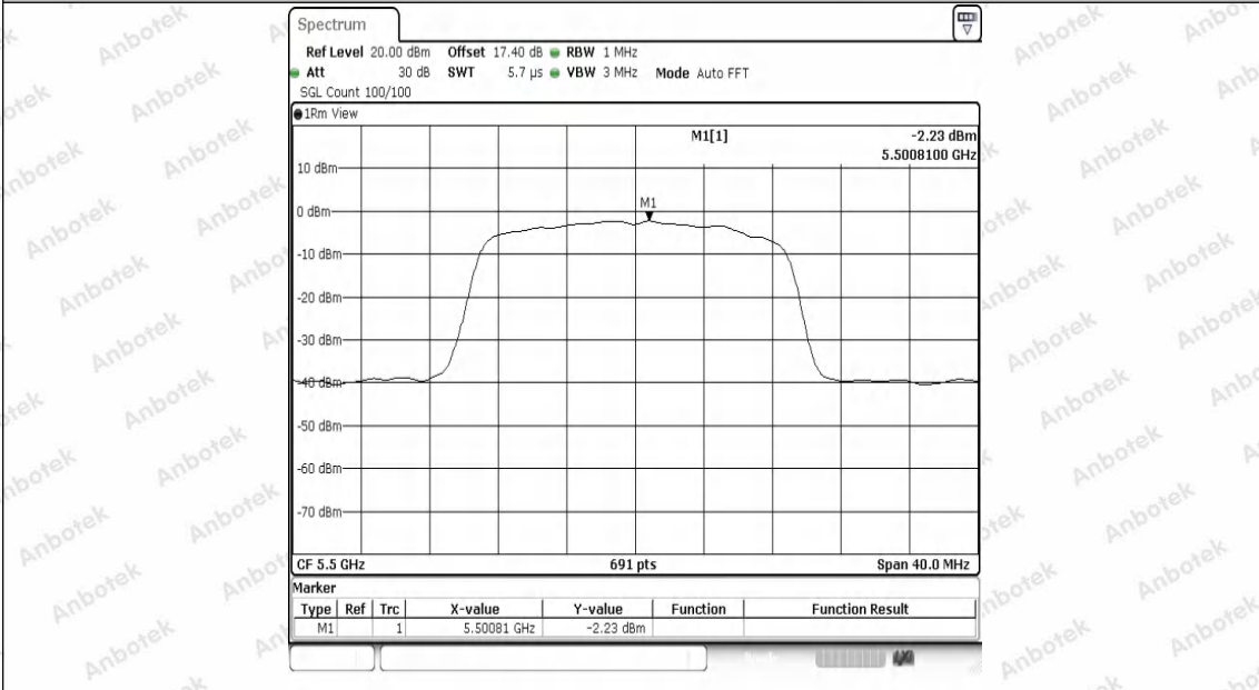
11AC20SISO-Ant1-5500-PASS
