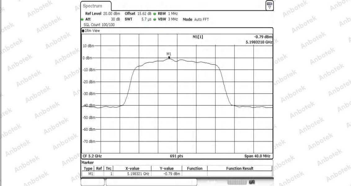
11N20SISO-Ant1-5200-PASS
