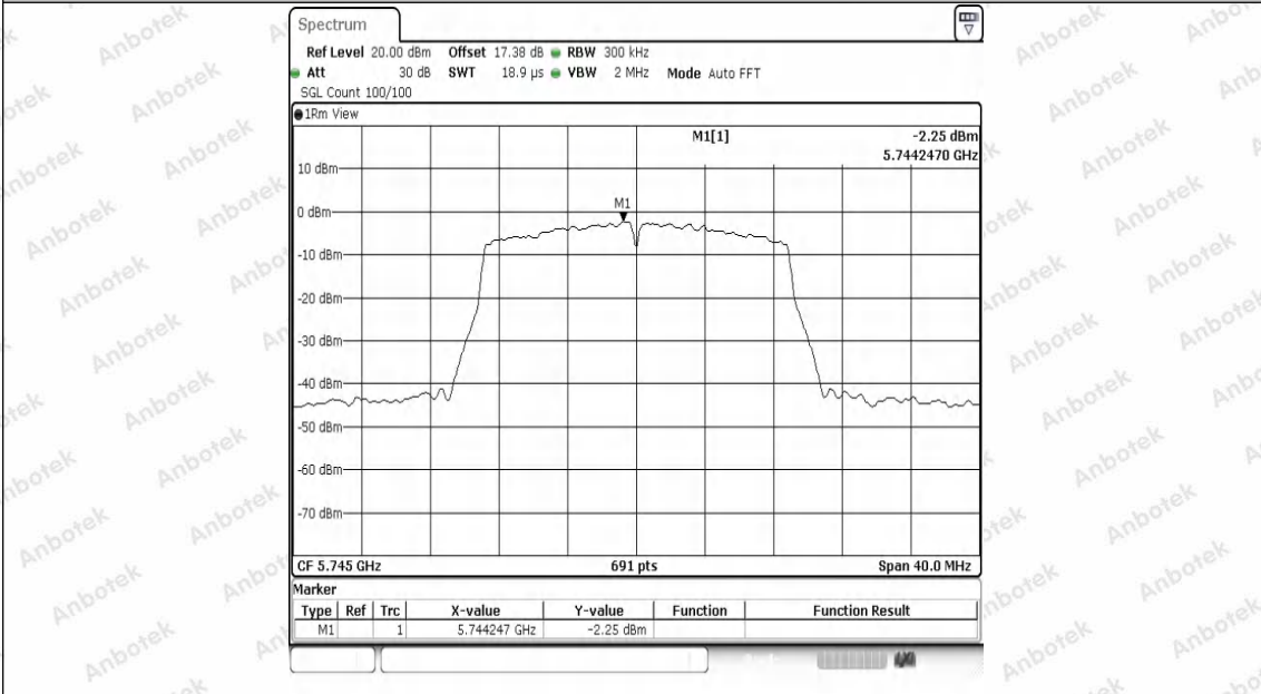
11N20SISO-Ant1-5745-PASS
