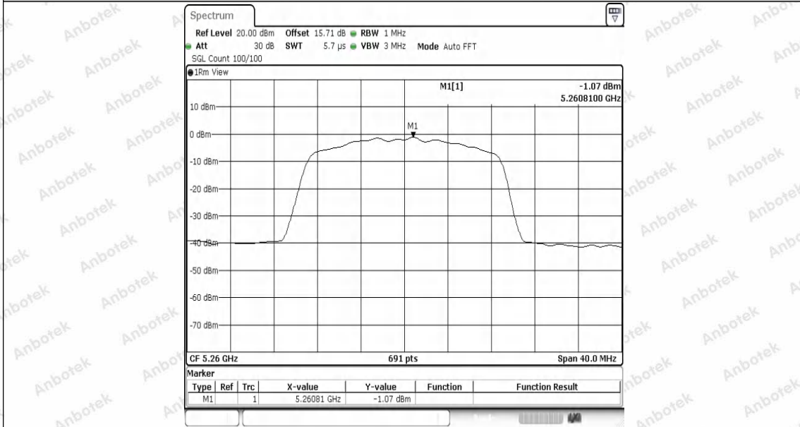
11N20SISO-Ant1-5260-PASS
