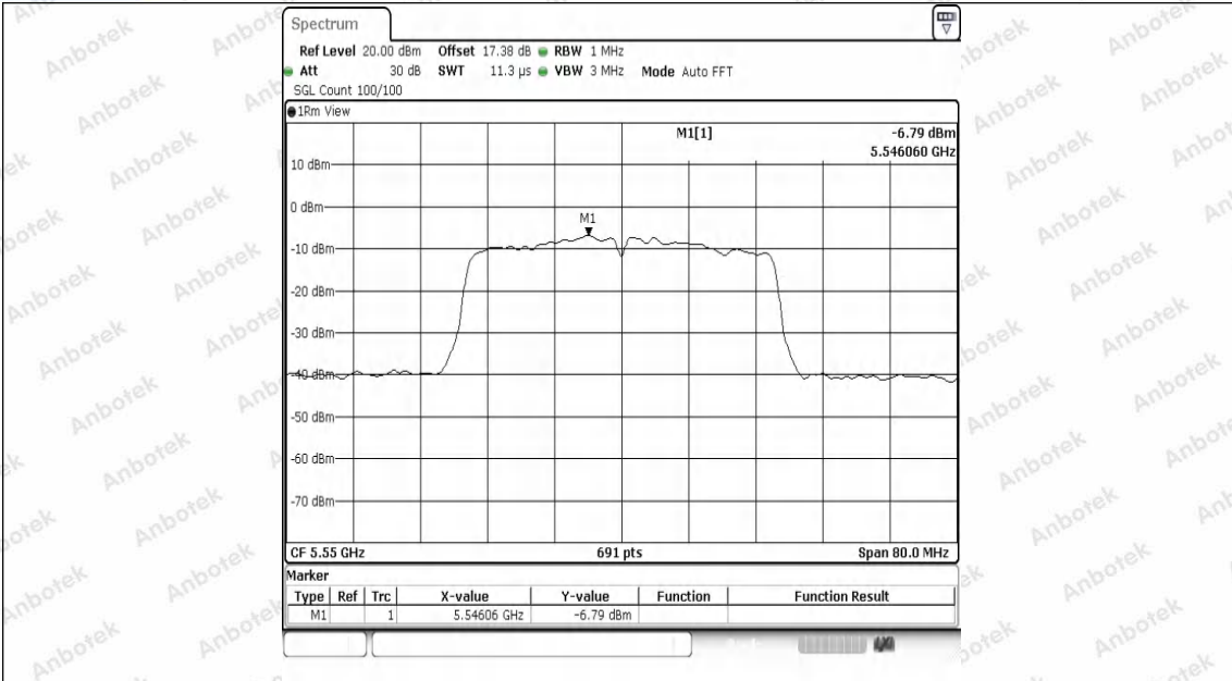
11AC40SISO-Ant1-5550-PASS
