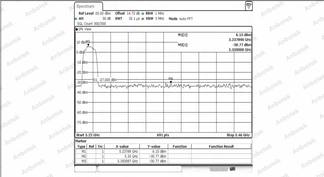
11N20SISO-Ant1-5240-PASS
