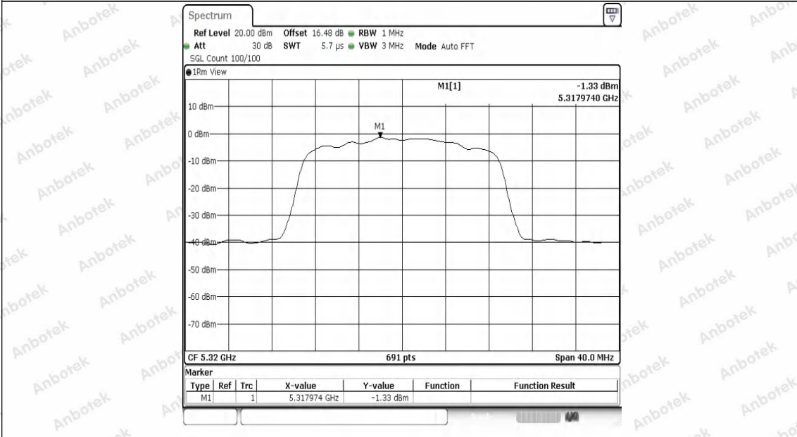
11N20SISO-Ant1-5320-PASS
