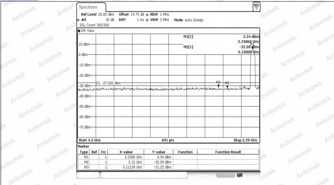
11N20SISO-Ant1-5260-PASS
