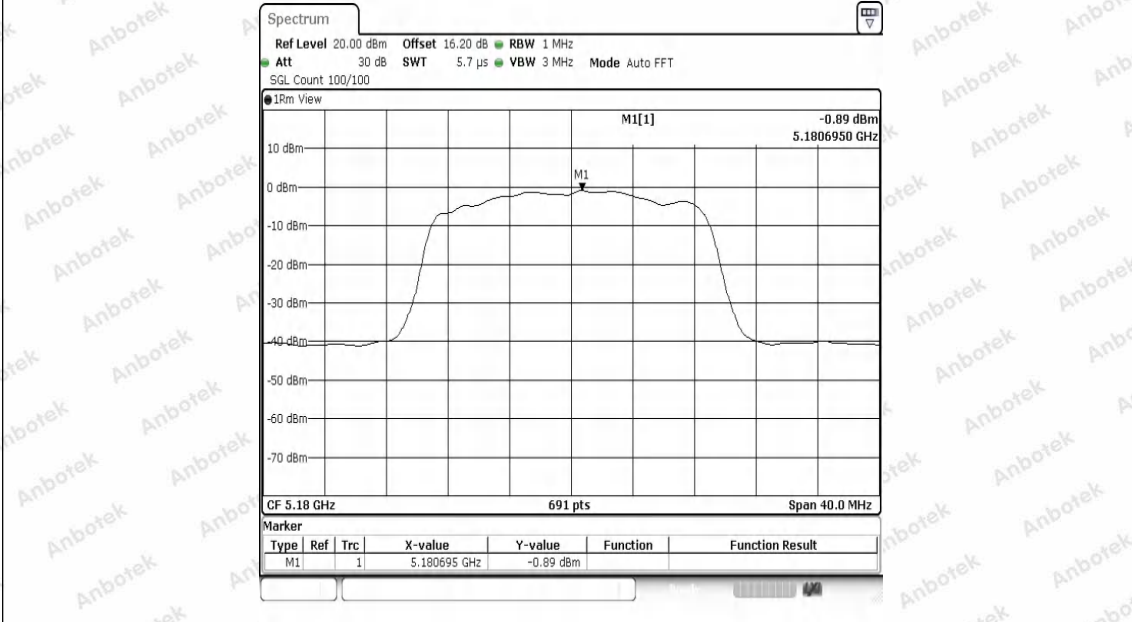
11AC20SISO-Ant1-5180-PASS
