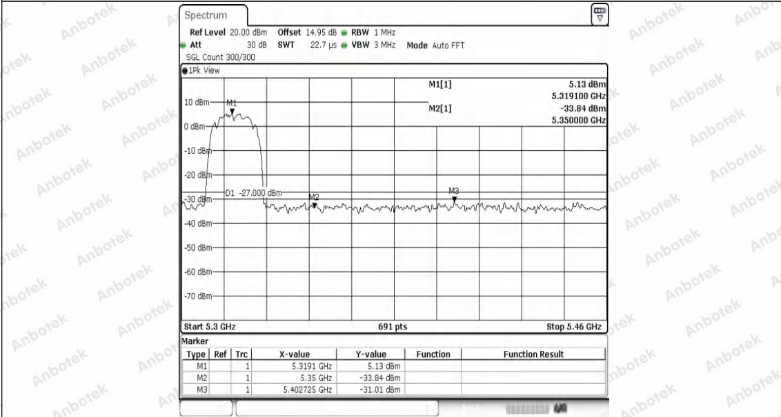
11N20SISO-Ant1-5320-PASS
