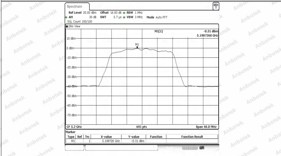
11A-Ant1-5200-PASS
