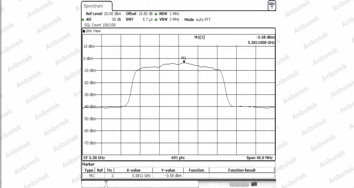
11N20SISO-Ant1-5580-PASS
