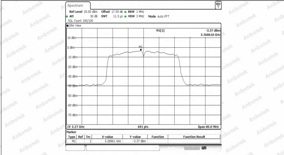
11AC40SISO-Ant1-5270-PASS
