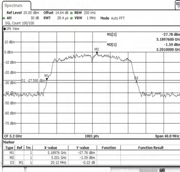
11N20SISO-Ant1-5200
