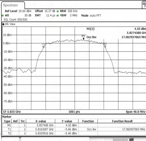
11A-Ant1-5825
