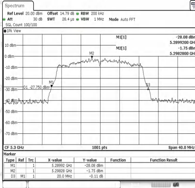
11N20SISO-Ant1-5300
