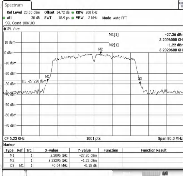
11N40SISO-Ant1-5230
