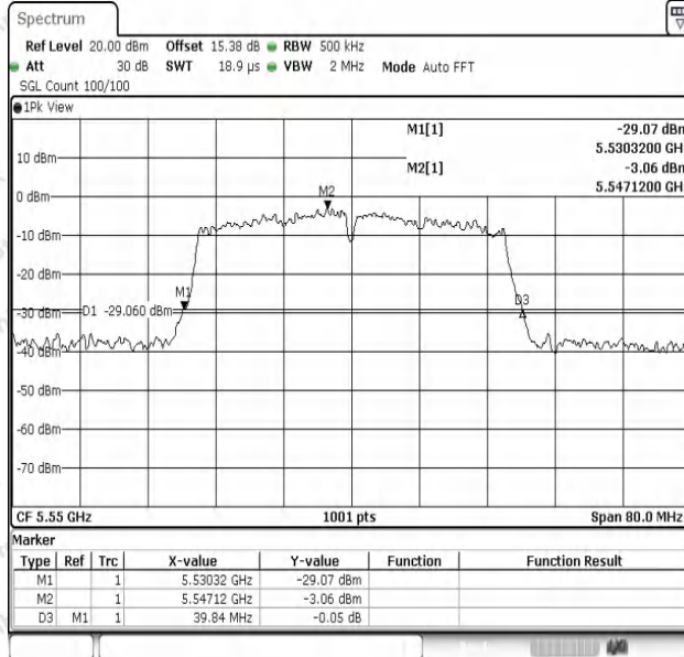
11N40SISO-Ant1-5550
