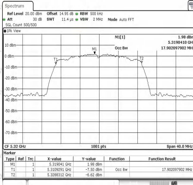
11N20SISO-Ant1-5320
