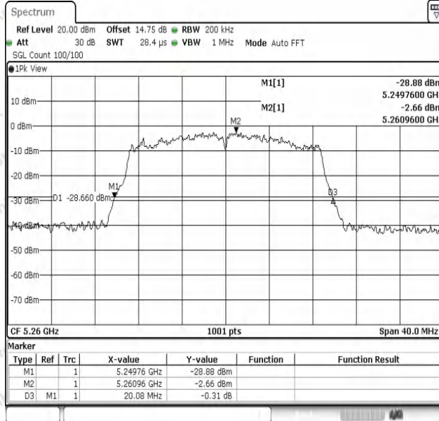
11N20SISO-Ant1-5260
