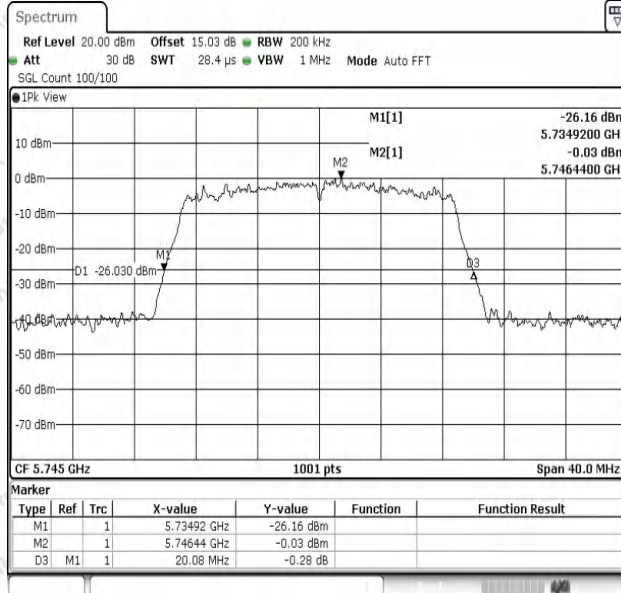
11N20SISO-Ant1-5745
