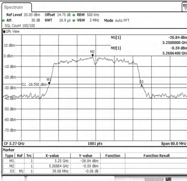
11AC40SISO-Ant1-5270
