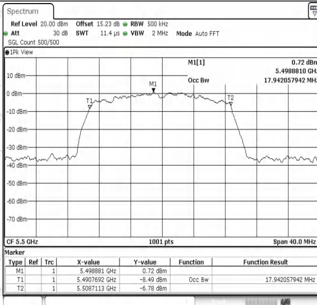
11AC20SISO-Ant1-5500
