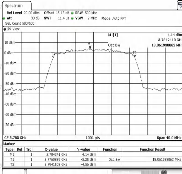
11AC20SISO-Ant1-5785
