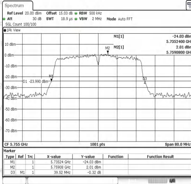
11AC40SISO-Ant1-5755
