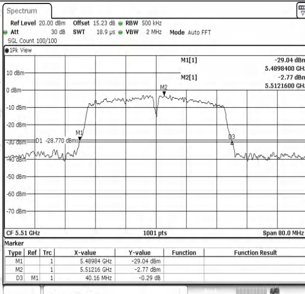
11AC40SISO-Ant1-5510
