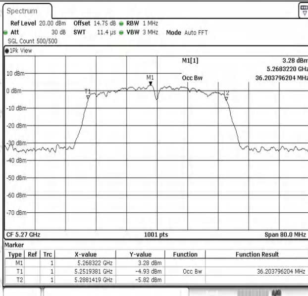
11AC40SISO-Ant1-5270
