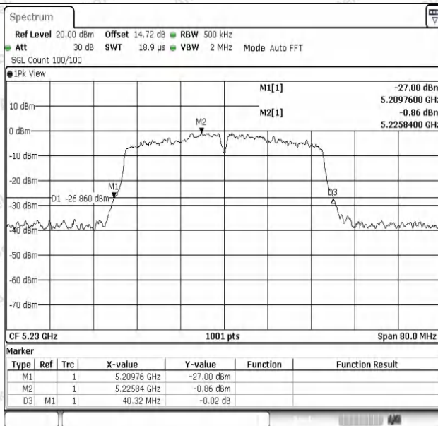
11AC40SISO-Ant1-5230
