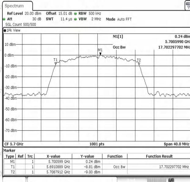
11AC20SISO-Ant1-5700
