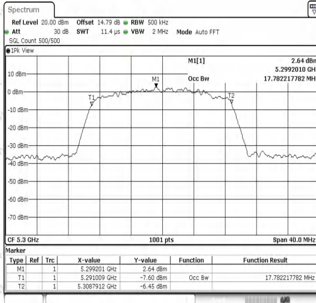
11AC20SISO-Ant1-5300
