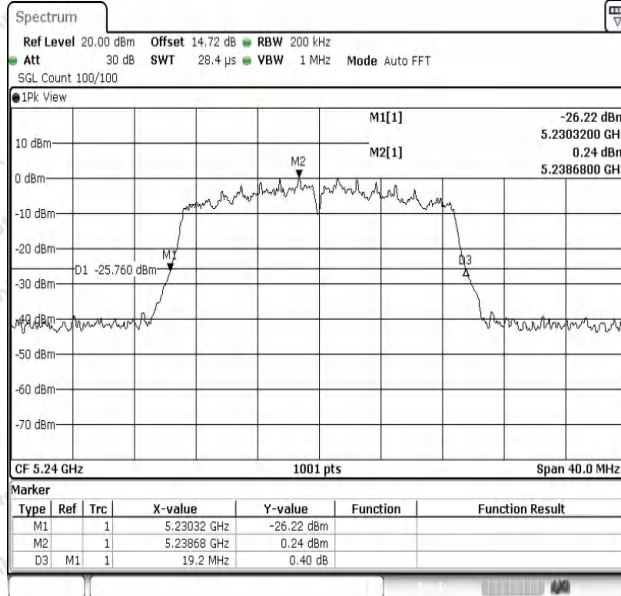
11AC20SISO-Ant1-5240
