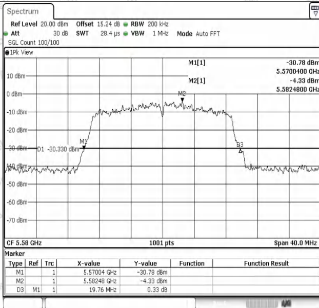
11AC20SISO-Ant1-5580
