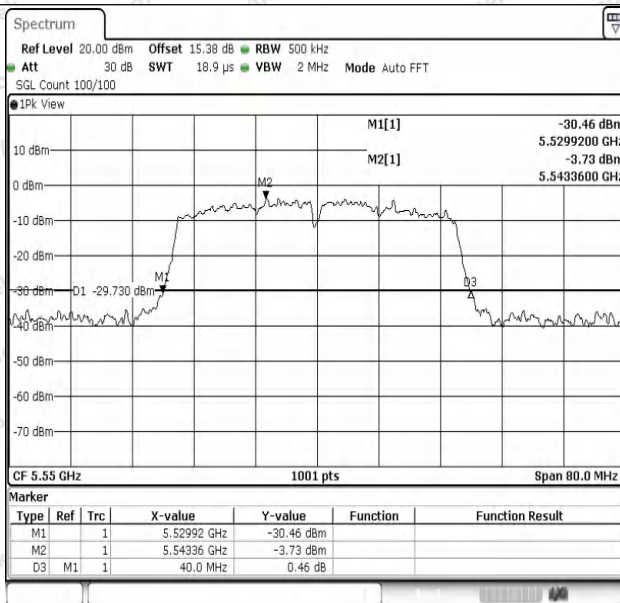
11AC40SISO-Ant1-5550
