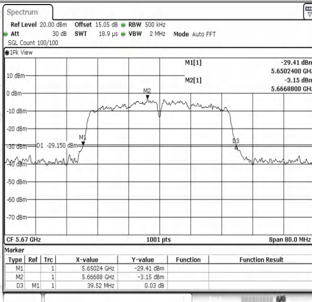
11AC40SISO-Ant1-5670
