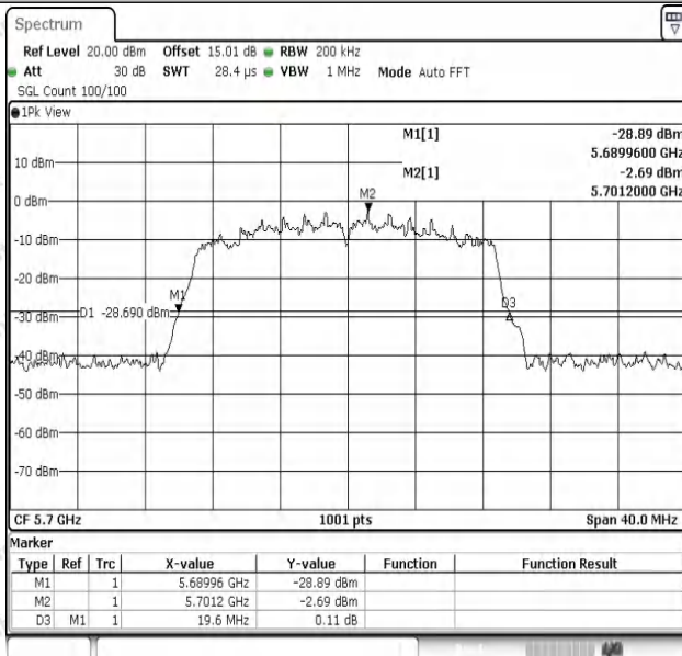
11AC20SISO-Ant1-5700
