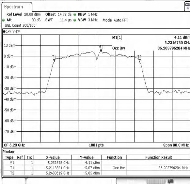
11AC40SISO-Ant1-5230
