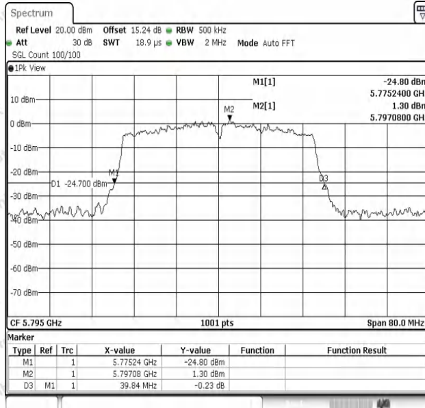
11AC40SISO-Ant1-5795
