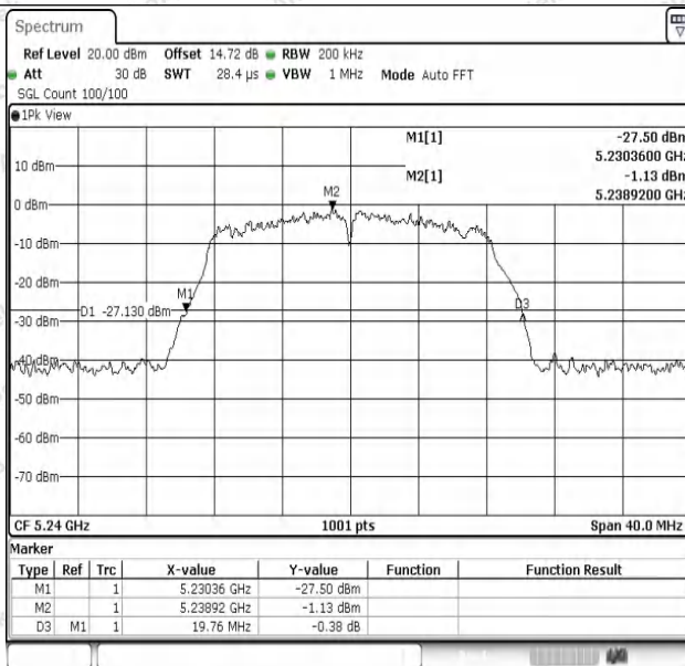
11A-Ant1-5240
