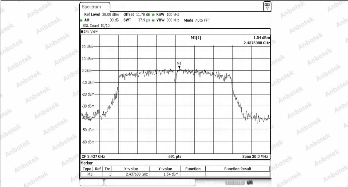
11N20SISO-Ant1-2437-0~Reference-PASS
