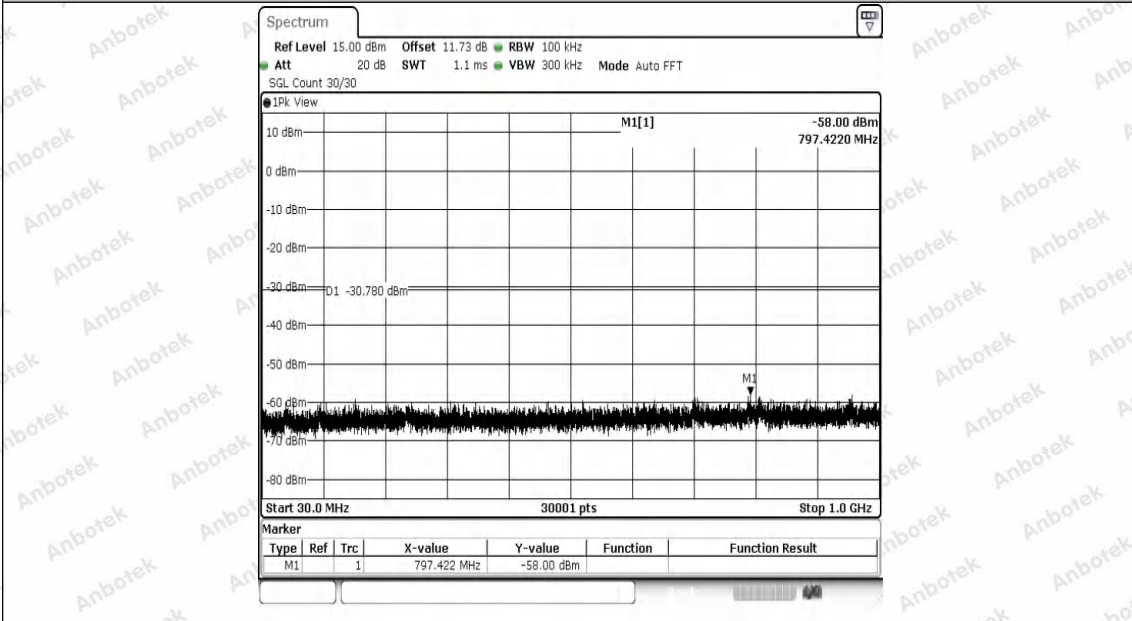
11N20SISO-Ant1-2462-30~1000-PASS
