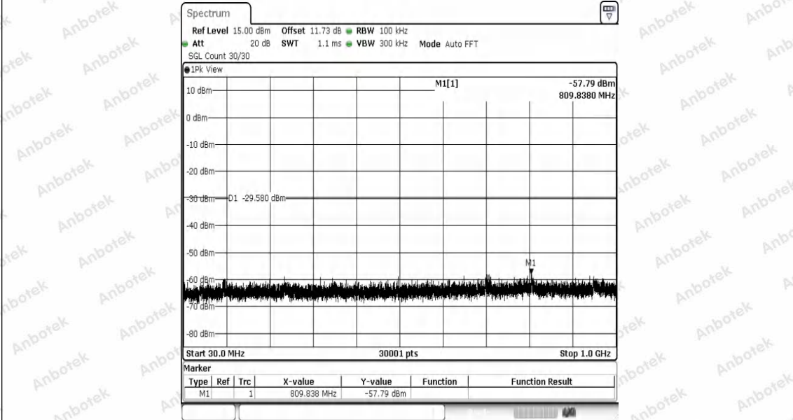
11B-Ant1-2462-30~1000-PASS
