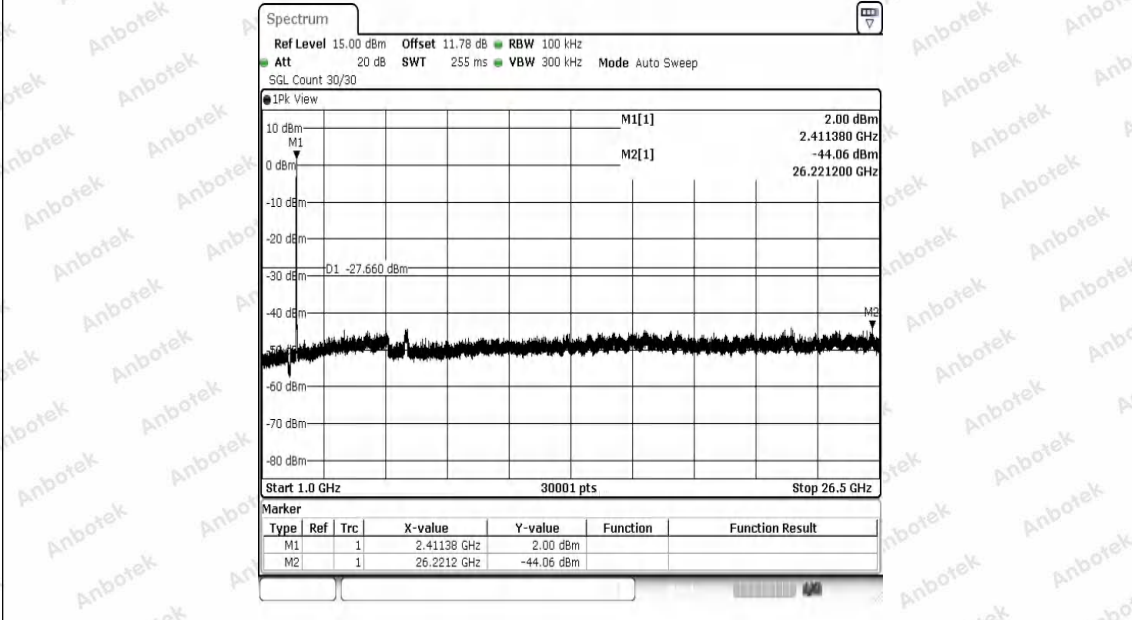
11G-Ant1-2412-1000~26500-PASS
