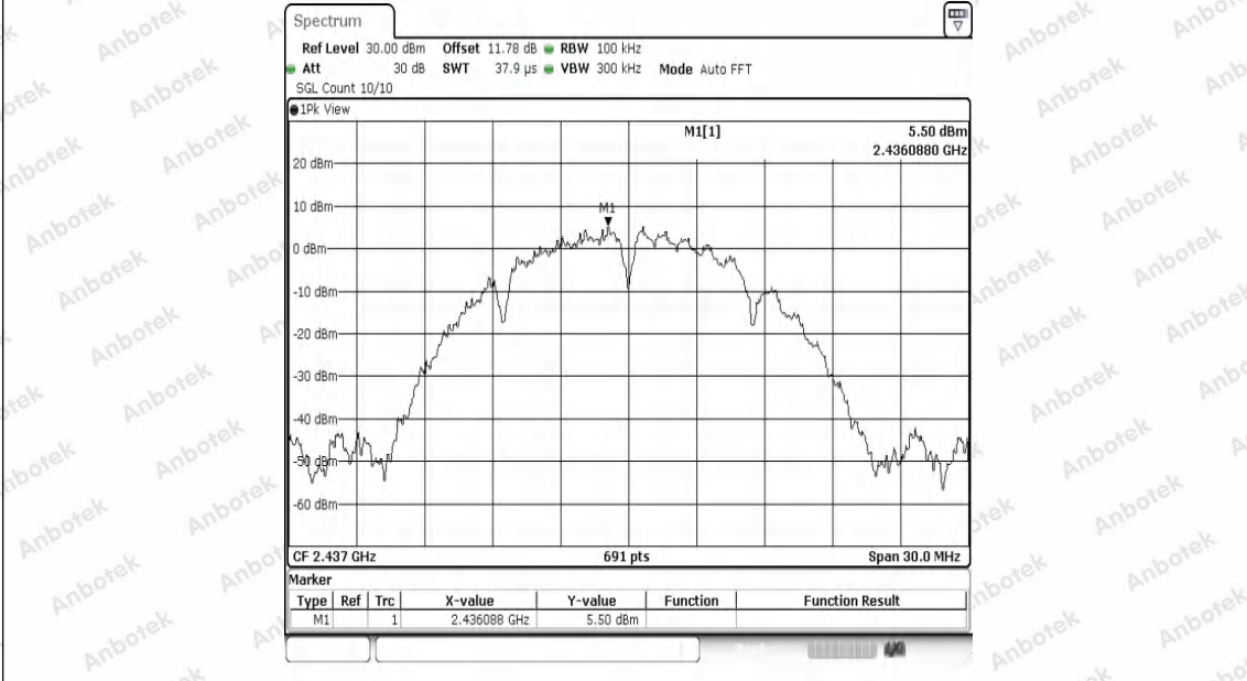
11B-Ant1-2437-0~Reference-PASS
