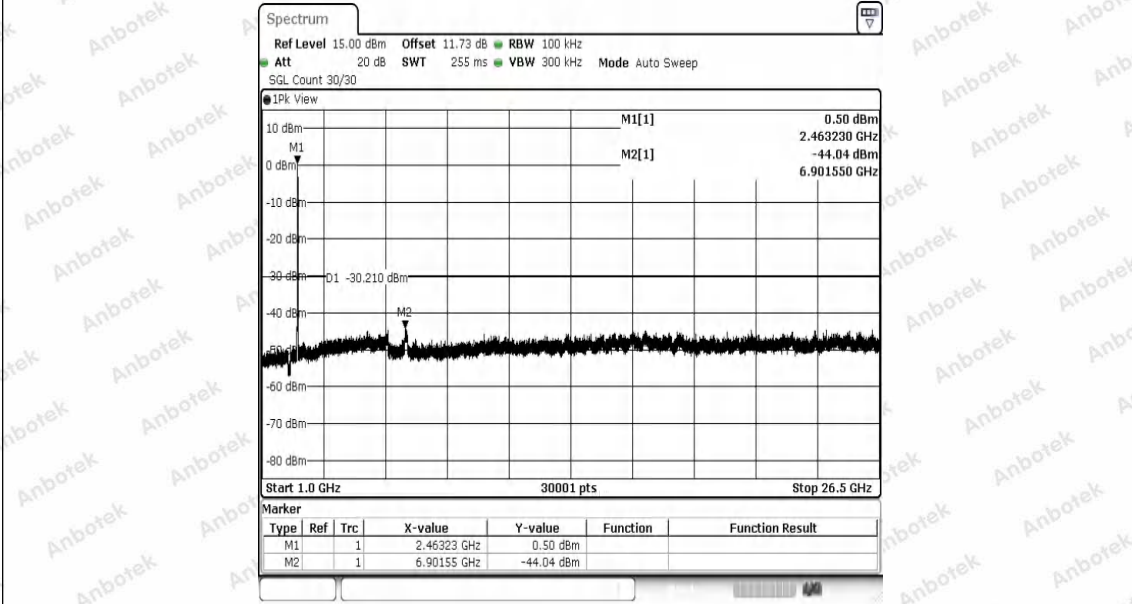
11G-Ant1-2462-1000~26500-PASS
