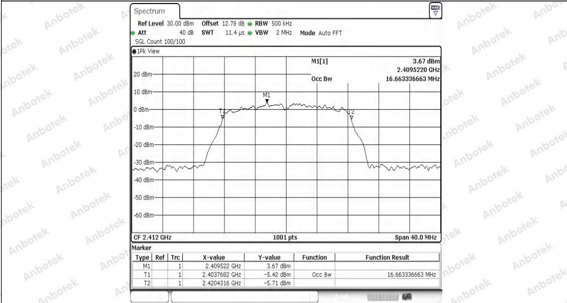
11G-Ant1-2412
