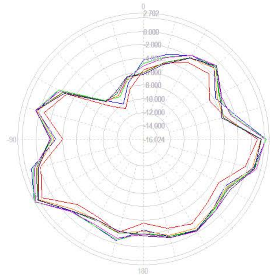
- E1 Plane Polar/Line Chart -
