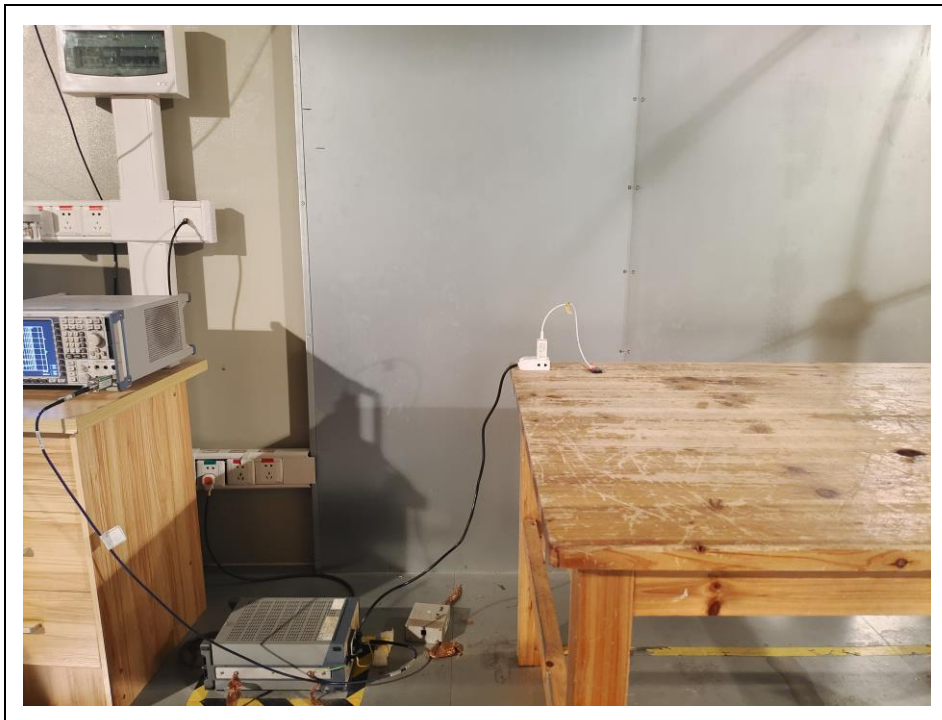
Conducted emissions
