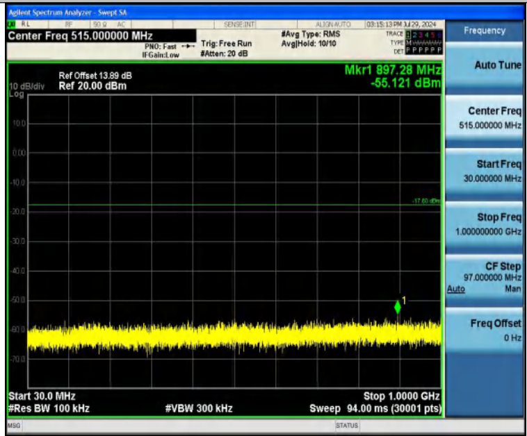
DH5-Ant1-2402-30~1000-PASS
