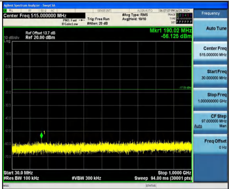
DH5-Ant1-2480-30~1000-PASS
