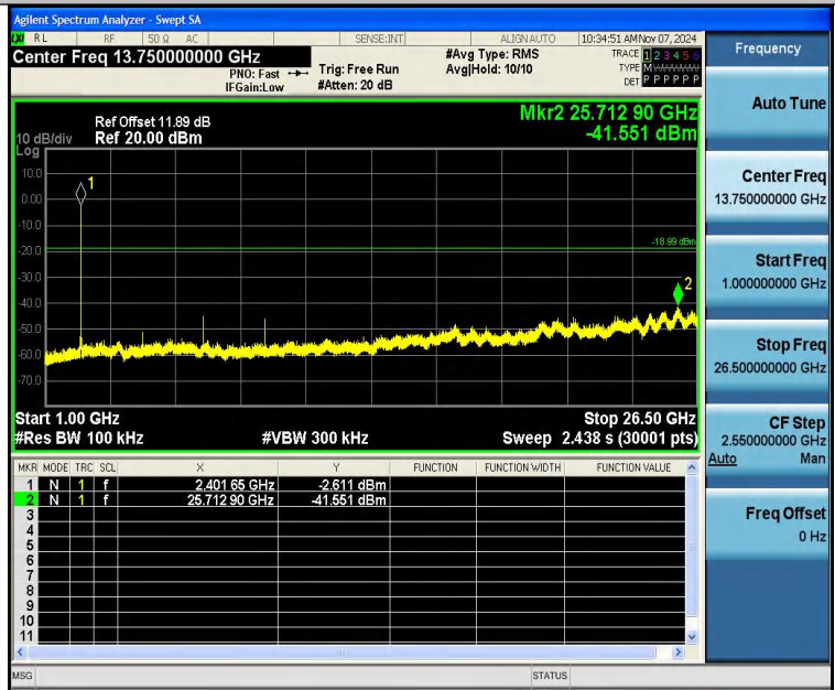
2DH5-Ant1-2402-1000~26500-PASS
