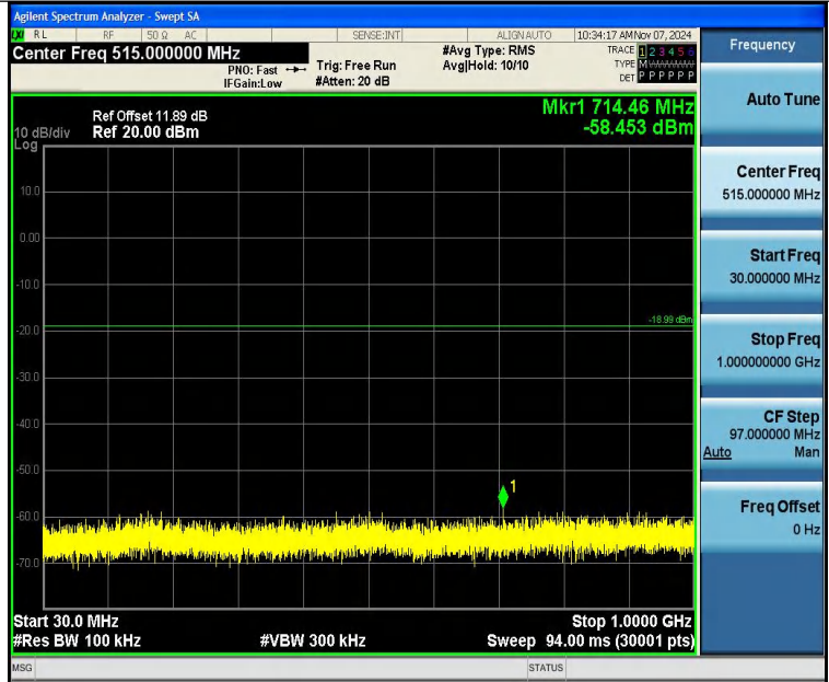
2DH5-Ant1-2402-30~1000-PASS
