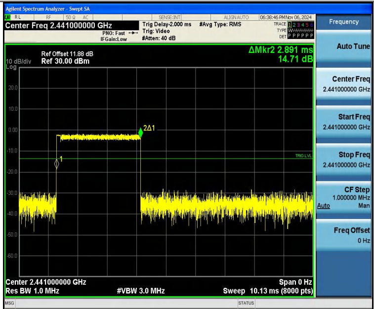
2DH5-Ant1-Hop-PASS
