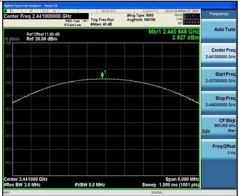
2DH5-Ant1-2441-PASS
