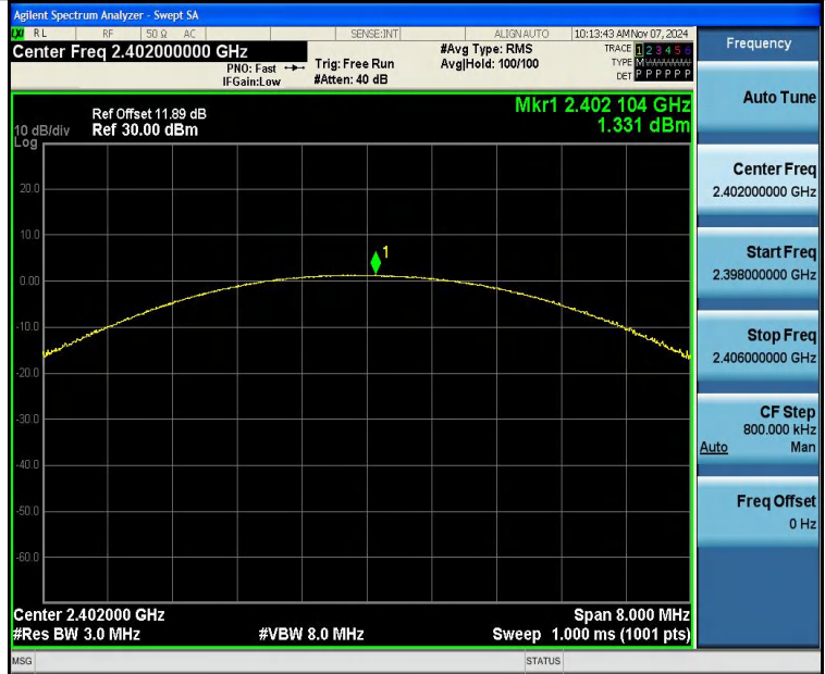
DH5-Ant1-2402-PASS
