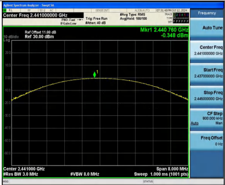
DH5-Ant1-2441-PASS
