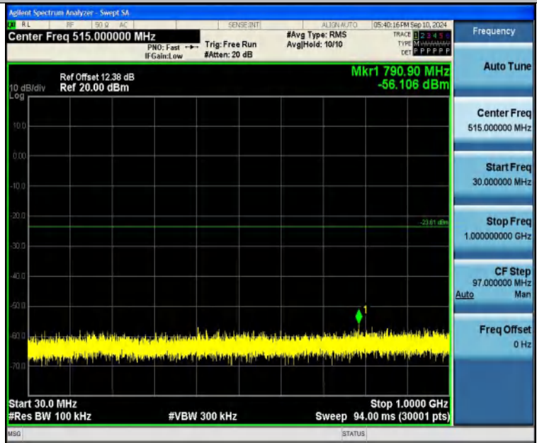
2DH5-Ant1-2441-30~1000-PASS
