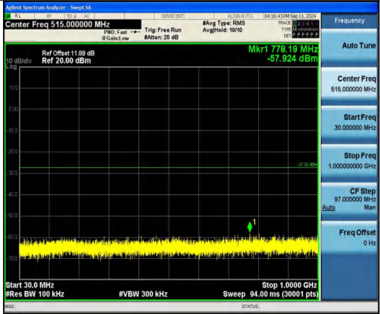
3DH5-Ant1-2402-30~1000-PASS
