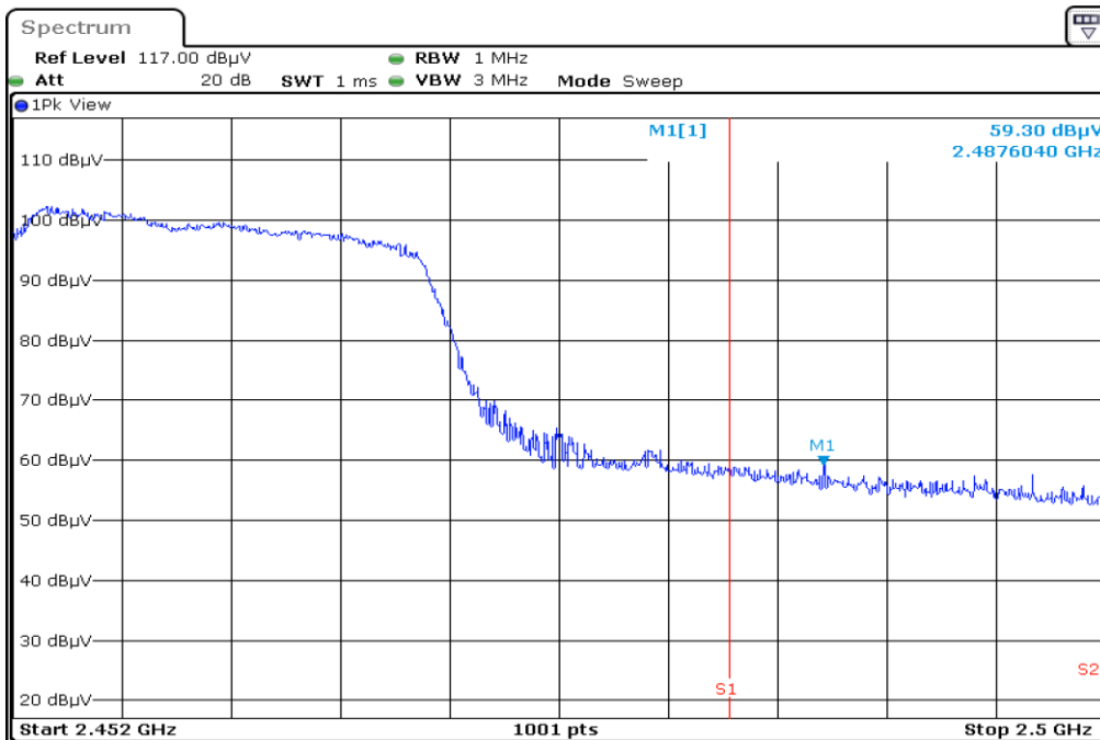
6 2452.0 F3 RestrictedBand Horizontal PEAK
