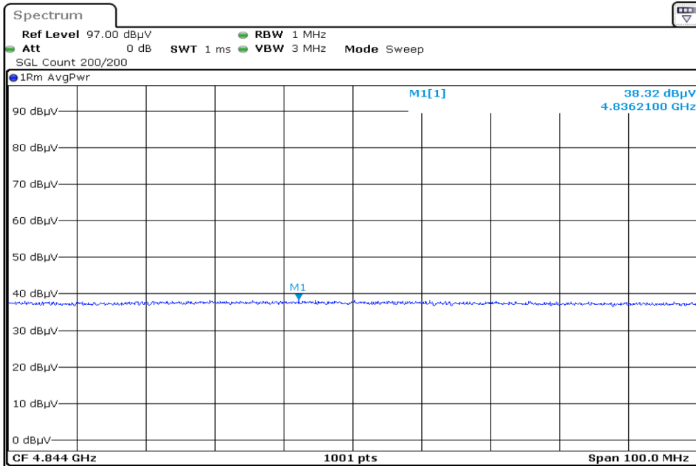
11 F1 X2 4844.0 Harmonic Vertical AVG
