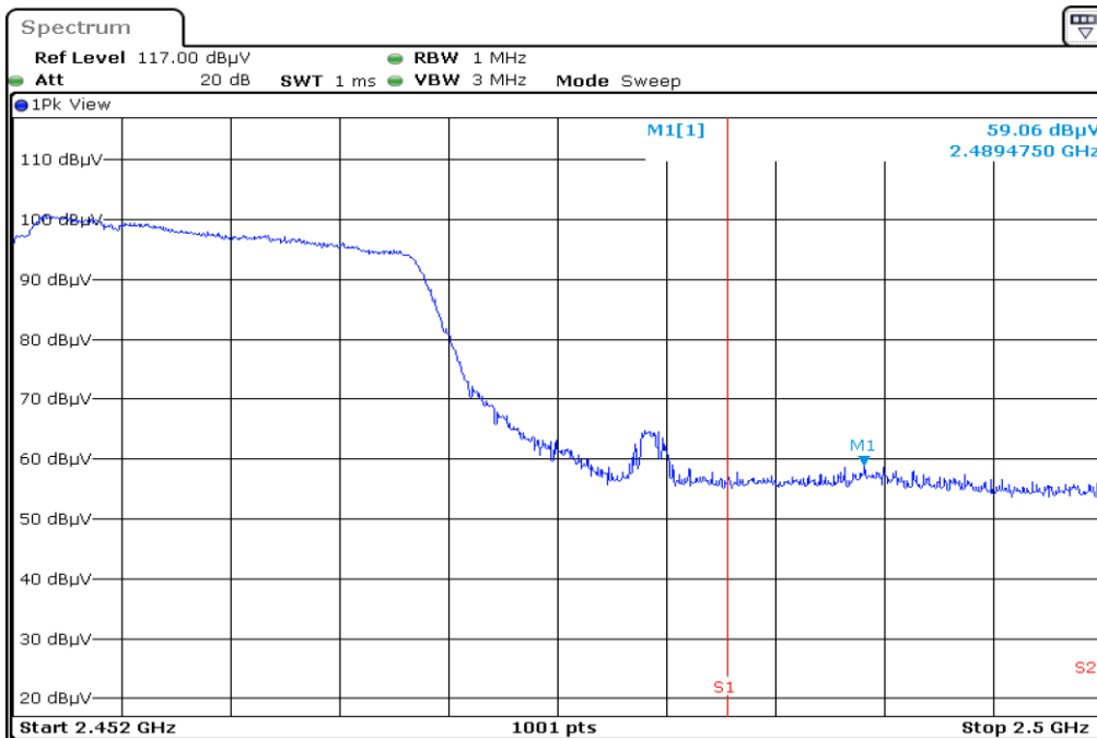
8 2452.0 F3 RestrictedBand Vertical PEAK
