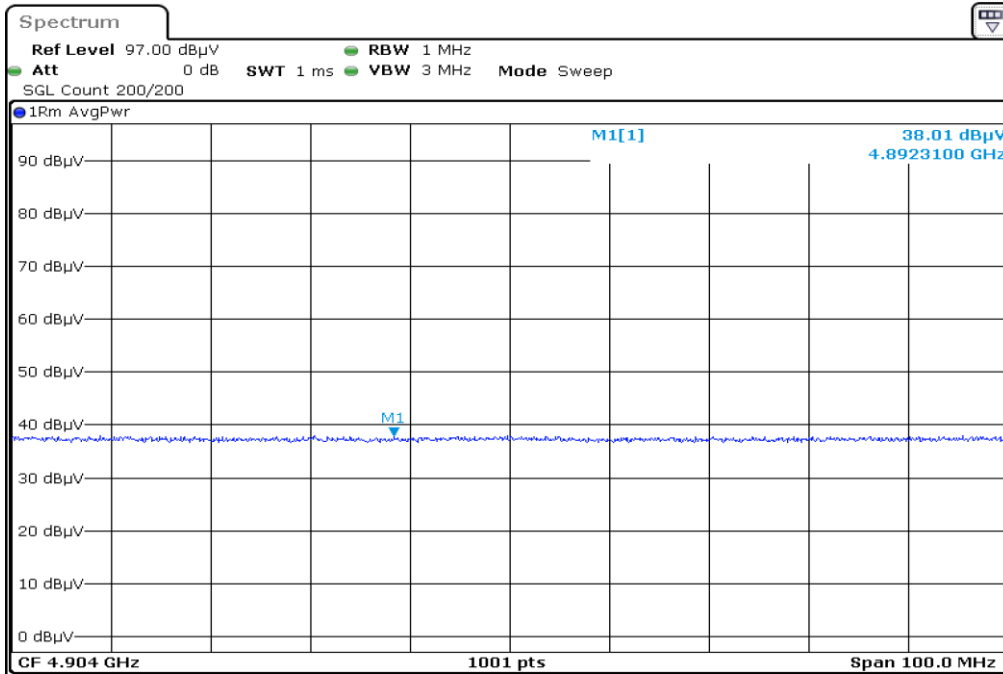
19 F3 X2 4904.0 Harmonic Vertical AVG
