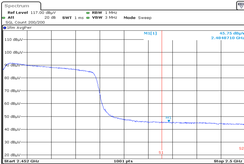
7 2452.0 F3 RestrictedBand Vertical AVG
