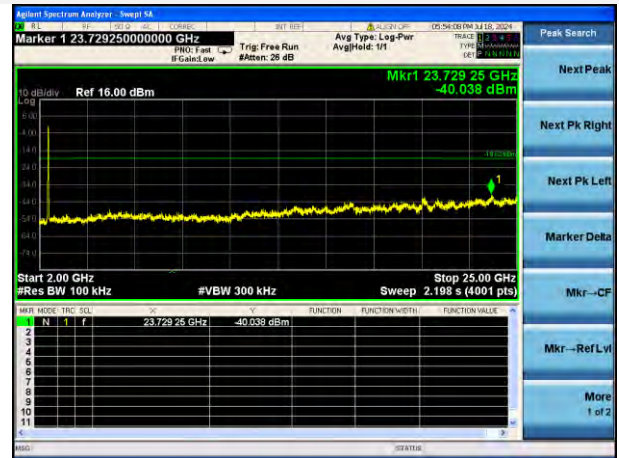
802.11n-40 MHz MIDDLE CHANNEL, SPURIOUS 2 GHz ~ 25 GHz
