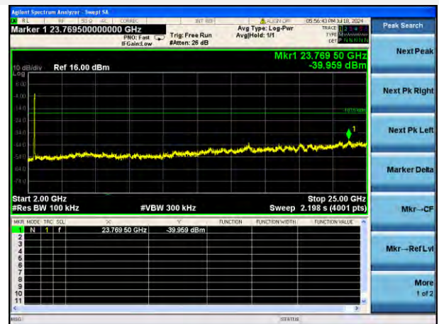
802.11n-40 MHz HIGH CHANNEL, SPURIOUS 2 GHz ~ 25 GHz
