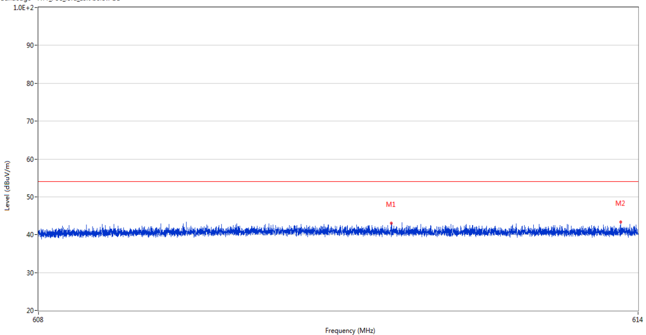
Bandedge - ATT_FCC_lora_Left below 1G
