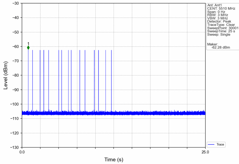
Signal Calibration_802.11ax(HEW40)_2C_5510MHz_RadarType6_Trial0
