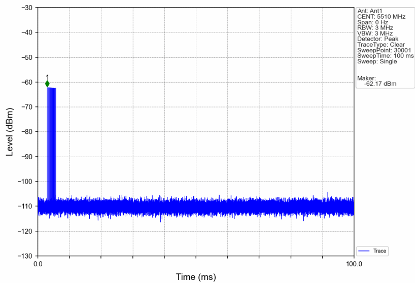
Signal Calibration_802.11ax(HEW40)_2C_5510MHz_RadarType6_Trial0
