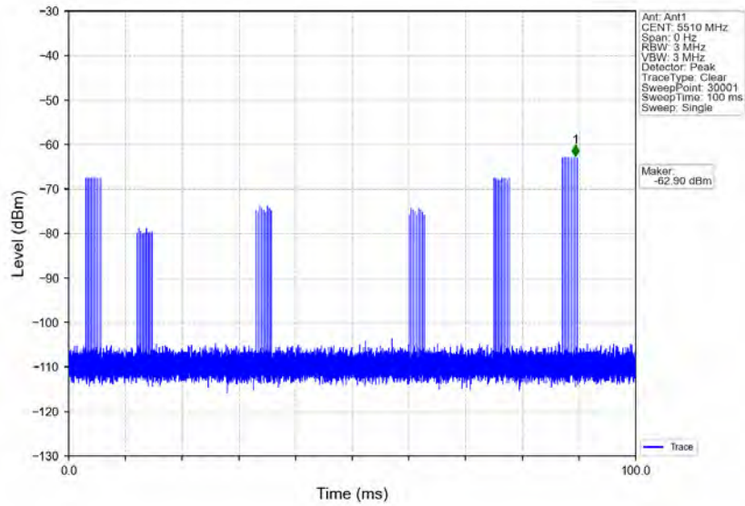
Signal Calibration 802.11ax(HEW40) 2C 5510MHz RadarType6 Trial0
