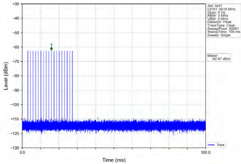
Signal Calibration 802.11ax(HEW40) 2C_5510MHz_RadarType1_Trial0
