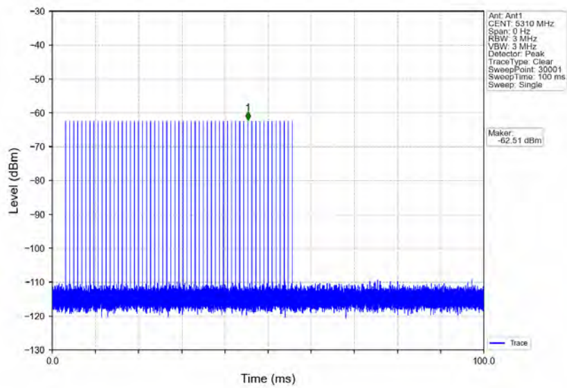
Signal Calibration 802.11ax(HEW40) 2A 5310MHz RadarType1 Trial0
