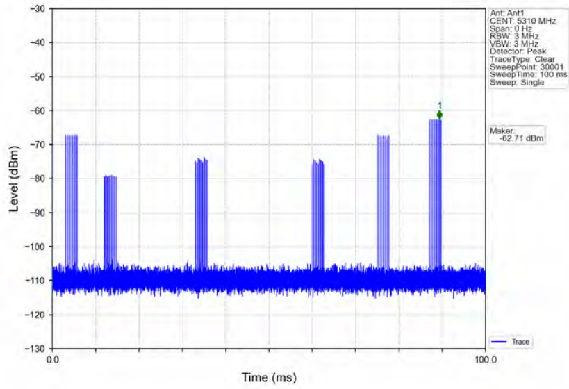
Signal Calibration 802.11ax(HEW40) 2A 5310MHz RadarType6 Trial0
