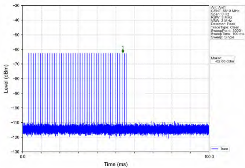
Signal Calibration 802.11ax(HEW40) 2C_5510MHz_RadarType1_Trial0
