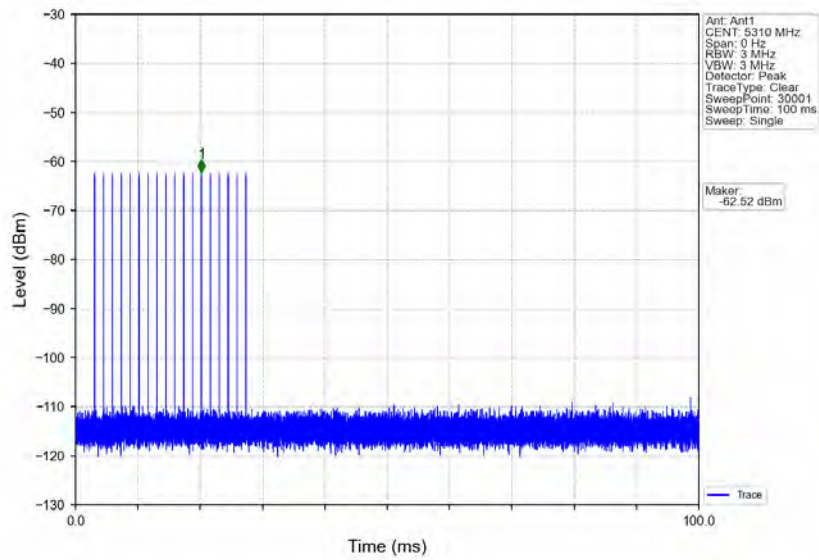
Signal Calibration 802.11ax(HEW40) 2A 5310MHz RadarType1 Trial0
