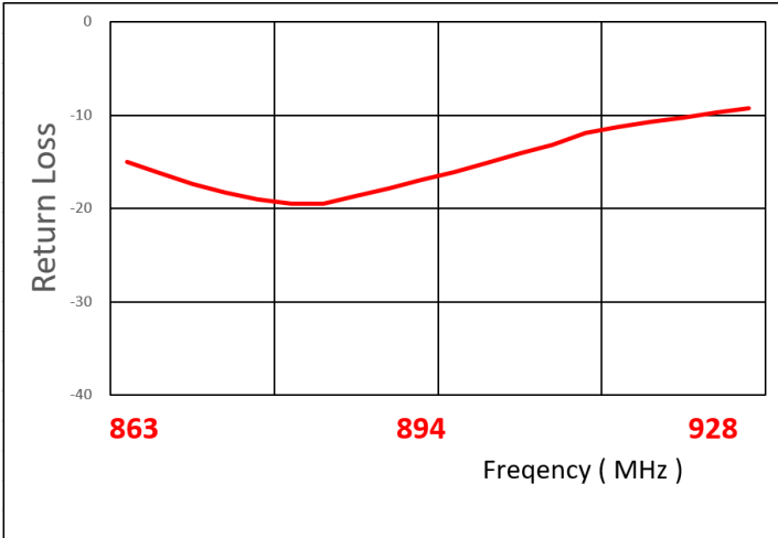
Return Loss
