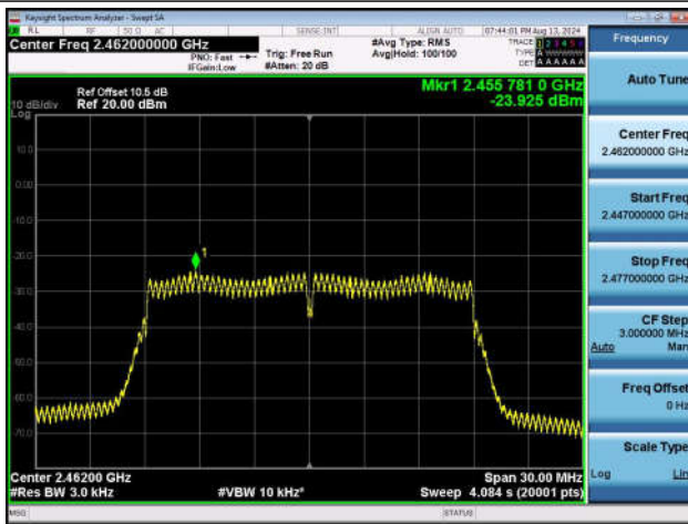
11N20SISO-Ant1-2462-PASS
