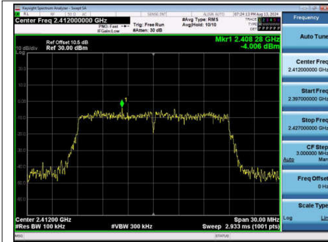
11N20SISO-Ant1-2412-0~Reference-PASS
