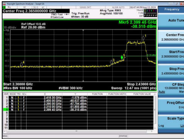
11G-Ant1-2412-PASS
