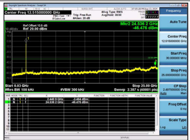
11G-Ant1-2437-30~25000-PASS
