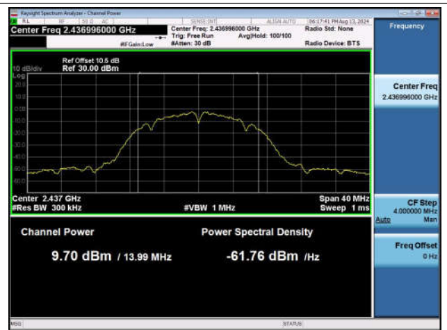
11B-Ant1-2437-PASS
