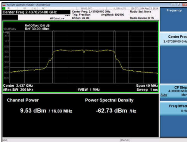
11G-Ant1-2437-PASS
