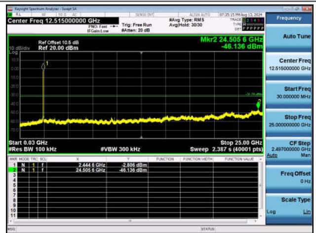
11N20SISO-Ant1-2437-30~25000-PASS
