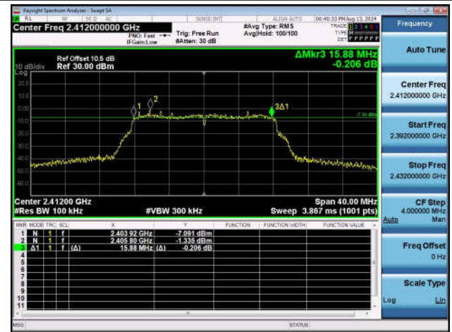
11G-Ant1-2412-PASS
