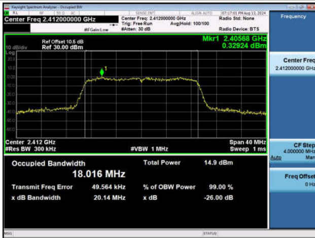
11N20SISO-Ant1-2412
