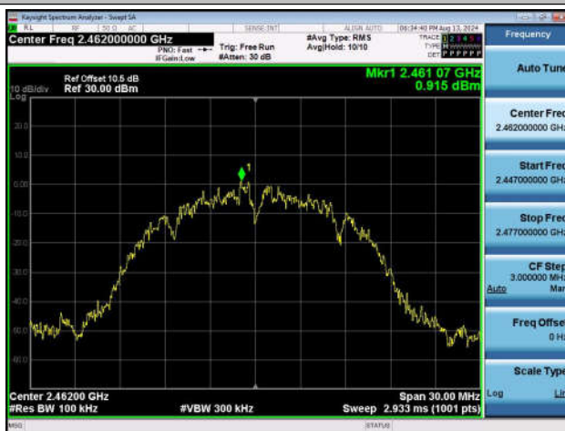
11B-Ant1-2462-0~Reference-PASS
