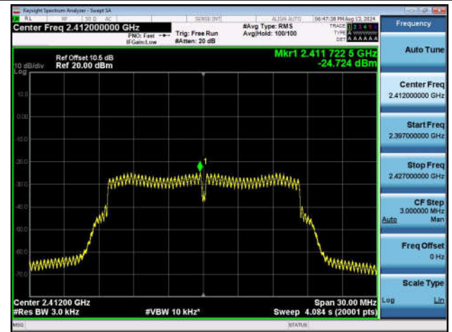
11G-Ant1-2412-PASS
