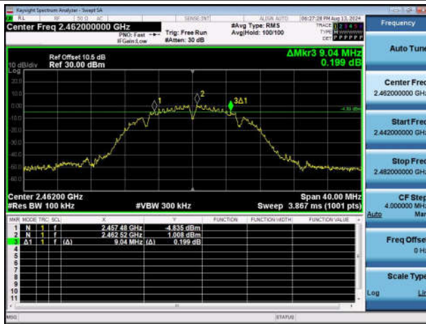
11B-Ant1-2462-PASS
