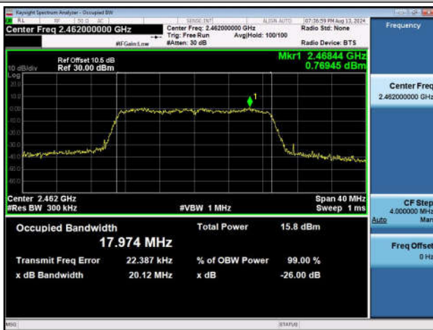
11N20SISO-Ant1-2462
