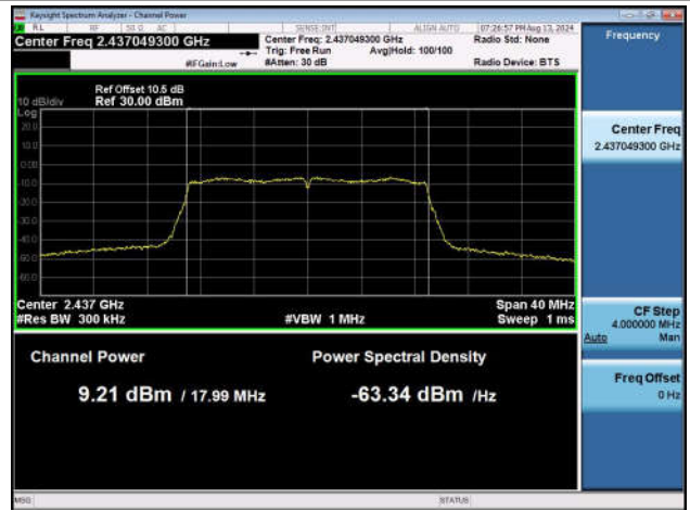
11N20SISO-Ant1-2437-PASS
