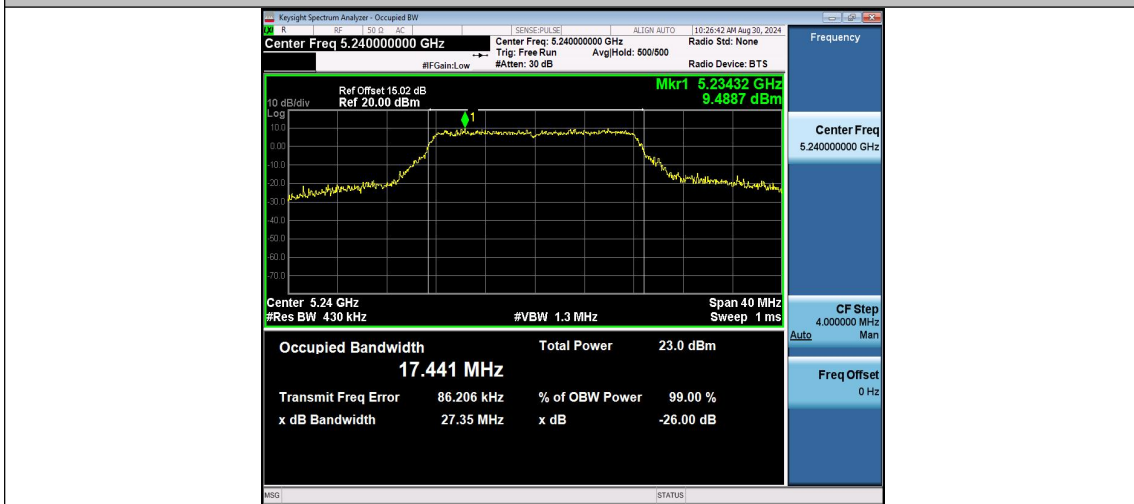
11A-Ant2-5240
