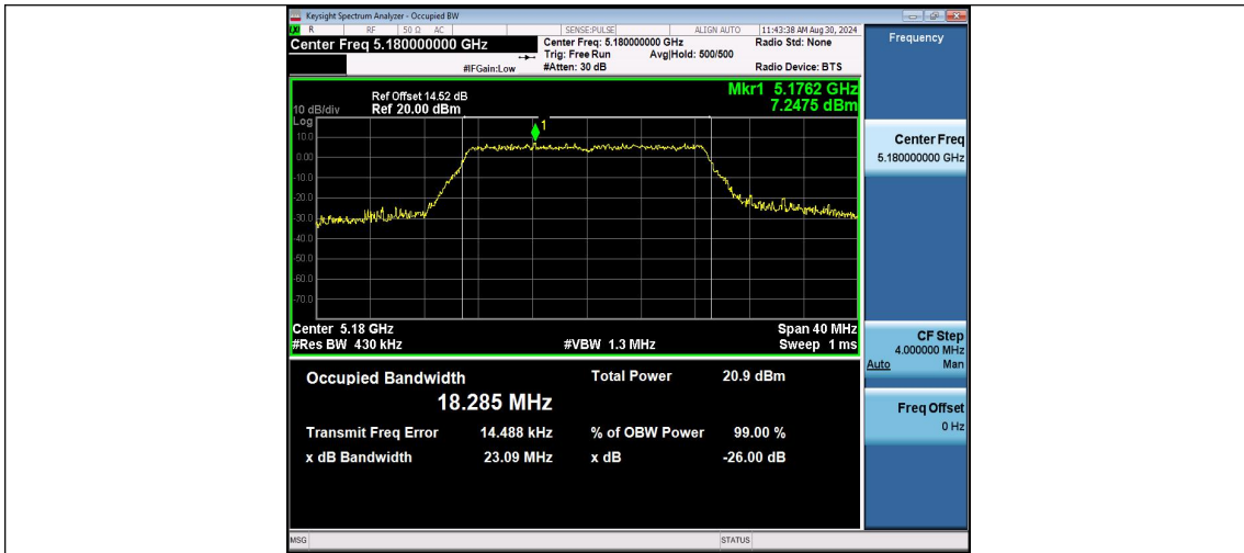
11N20MIMO-Ant1-5180
