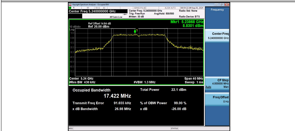
11A-Ant1-5240
