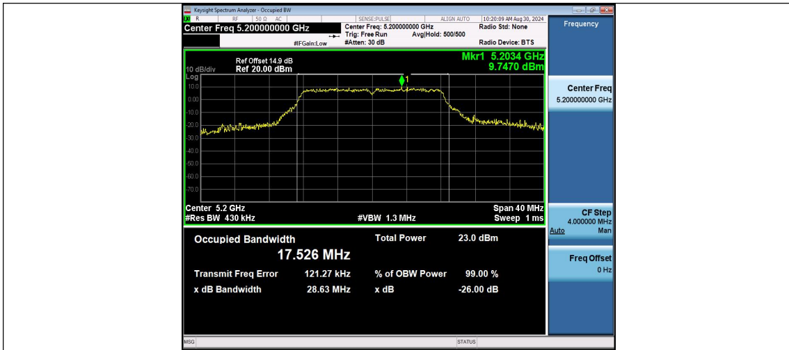
11A-Ant2-5200
