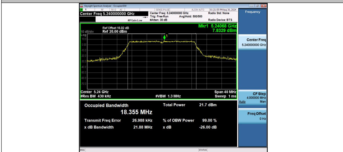
11N20MIMO-Ant2-5240
