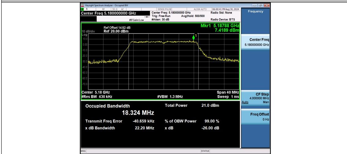
11AC20MIMO-Ant1-5180
