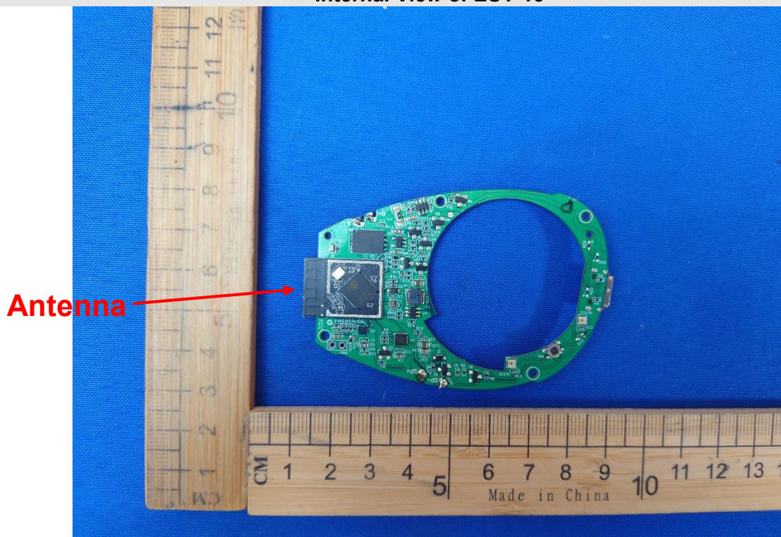
Internal View of EUT-13
