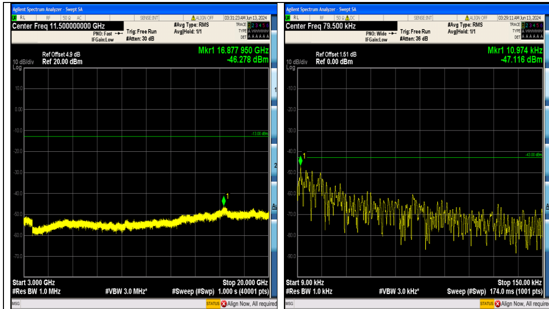
Band4_5MHz_QPSK_20375_25RB#0_3000~2000_3000~20000
