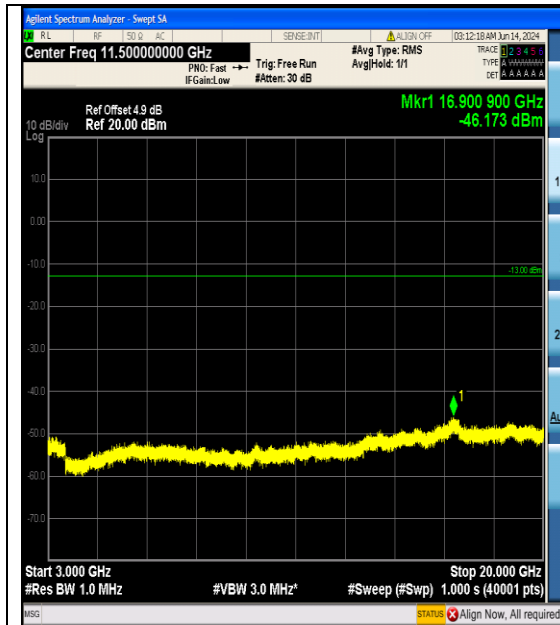
Band66_3MHz_16QAM_132322_15RB#0_3000 ~20000_3000~20000
