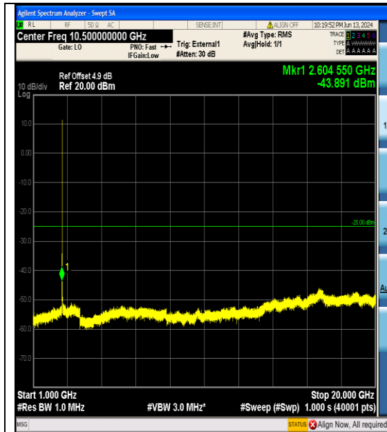
Band38_5MHz_16QAM_38225_25RB#0_1000~ 20000_1000~20000
