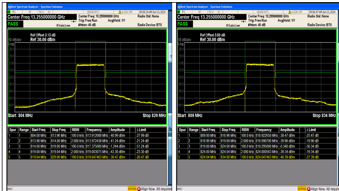
Band26_5MHz_QPSK_26715_25RB#0
