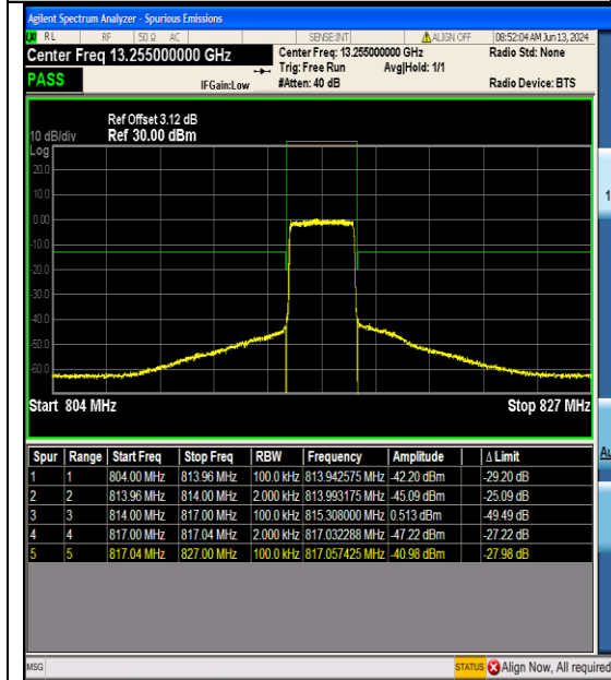
Band26_3MHz_16QAM_26705_15RB#0
