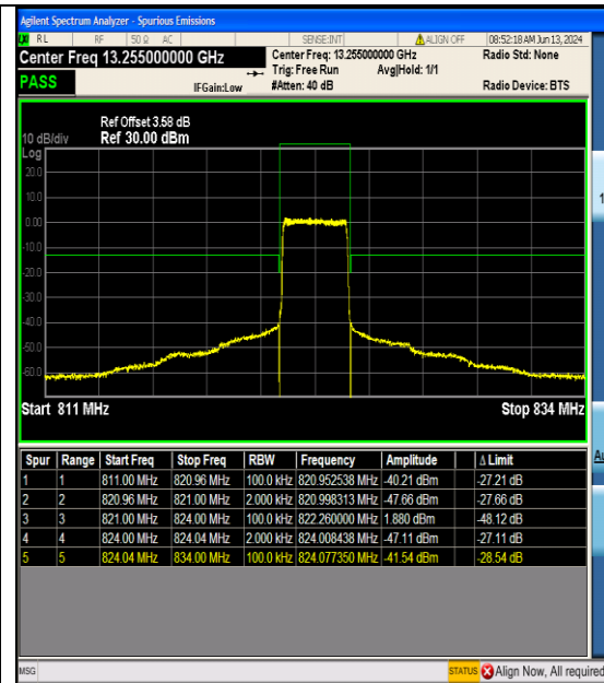
Band26_3MHz_QPSK_26775_15RB#0
