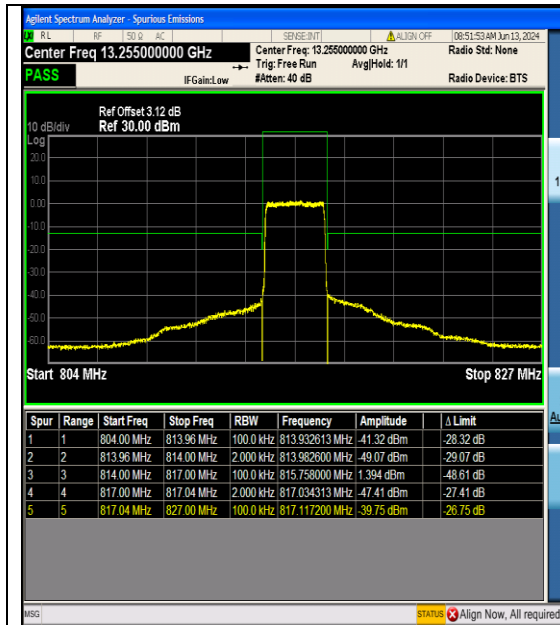
Band26_3MHz_QPSK_26705_15RB#0
