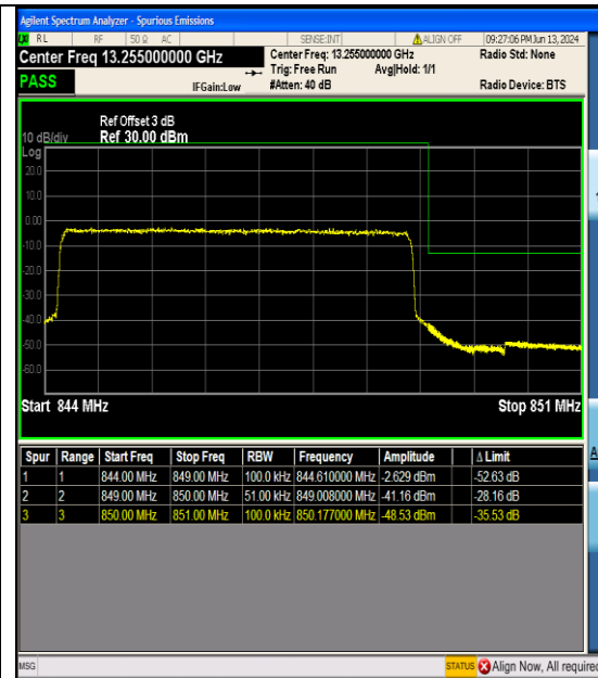
Band26_5MHz_16QAM_27015_25RB#0
