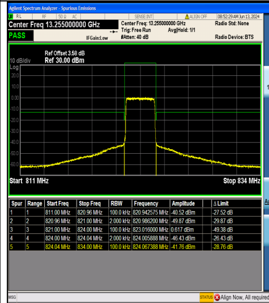
Band26_3MHz_16QAM_26775_15RB#0
