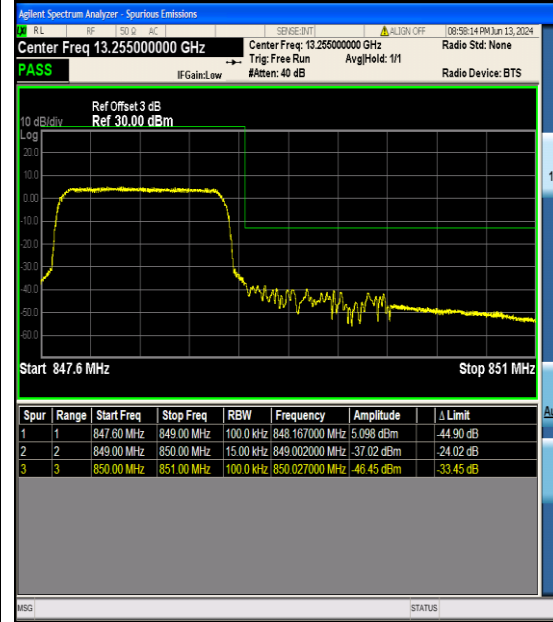
Band26_1.4MHz_QPSK_27033_6RB#0
