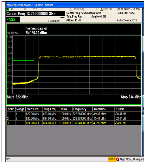
Band26_10MHz_16QAM_26840_50RB#0
