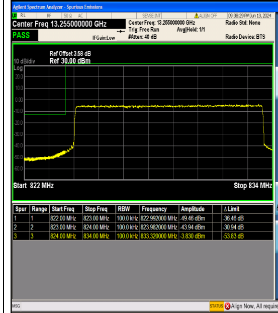
Band26_10MHz_QPSK_26840_50RB#0
