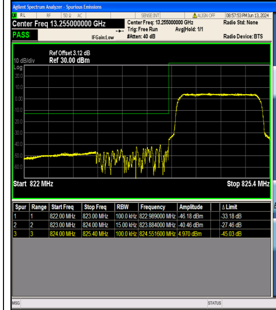
Band26_1.4MHz_QPSK_26797_6RB#0
