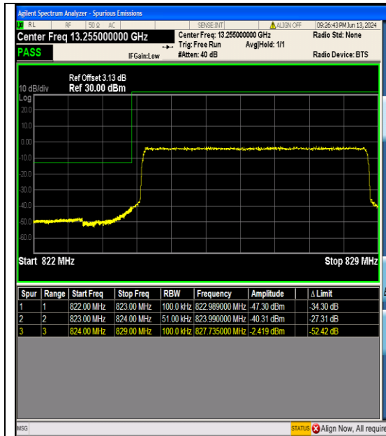
Band26_5MHz_16QAM_26815_25RB#0
