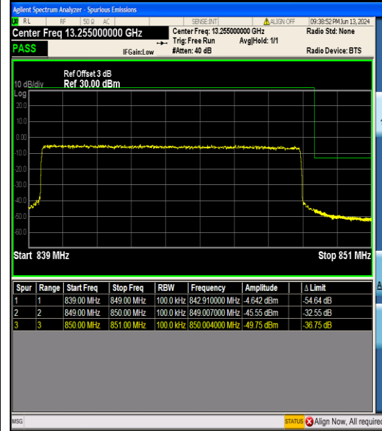
Band26_10MHz_QPSK_26990_50RB#0
