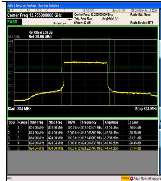
Band26_10MHz_QPSK_26740_50RB#0
