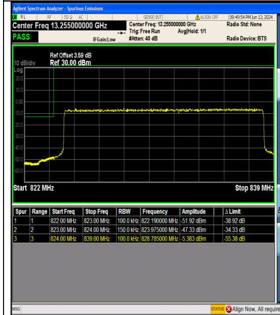
Band26_15MHz_QPSK_26865_75RB#0
