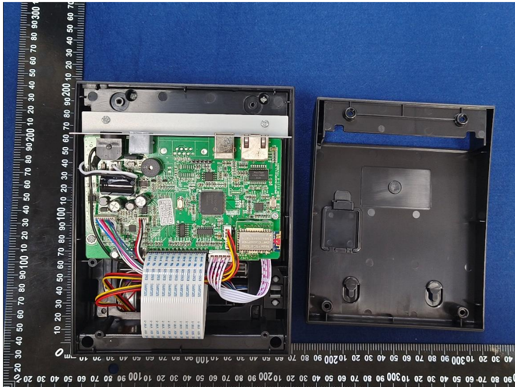
Internal Photo FCC ID: 2BHCJ-WPA1B
