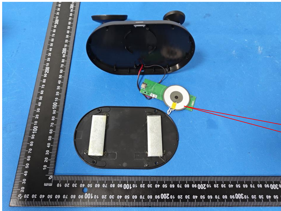
Antenna Earphone
