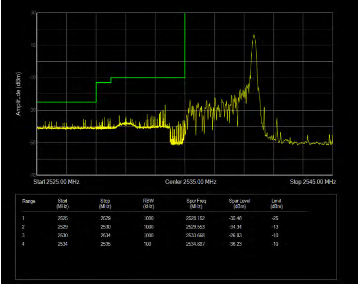
Band41(2535-2655) 16QAM BW=5MHz Channel=40065 RB Size=25 Position=#0 Extended
