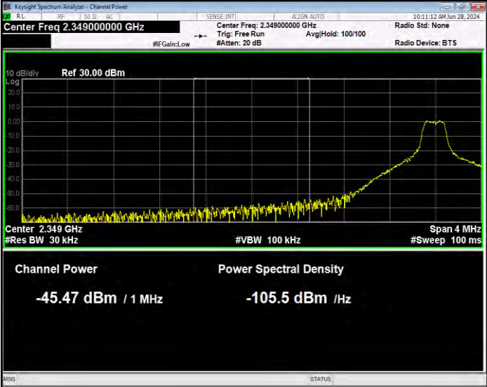
Band40(2350-2360) 16QAM BW=10MHz Channel=39200 RB Size=1 Position=#0 Normal
