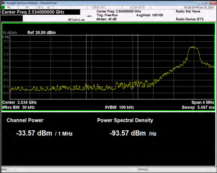
Band41(2535-2655) 16QAM BW=10MHz Channel=40090 RB Size=1 Position=#0 Normal
