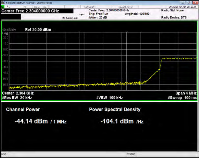
Band40(2305-2315) 16QAM BW=5MHz Channel=38725 RB Size=25 Position=#0 Normal
