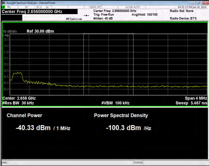
Band41(2535-2655) 16QAM BW=15MHz Channel=41165 RB Size=1 Position=#0 Normal
