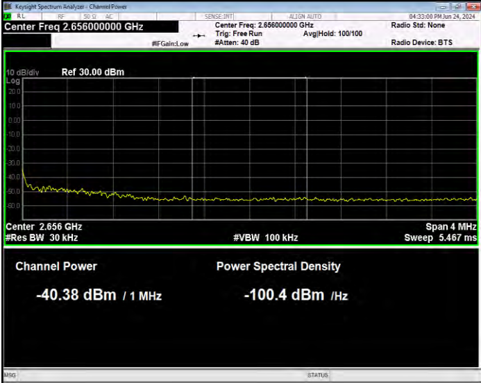
Band41(2535-2655) 16QAM BW=20MHz Channel=41140 RB Size=1 Position=#0 Normal
