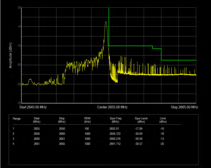
Band41(2535-2655) 16QAM BW=5MHz Channel=41215 RB Size=25 Position=#0 Extended
