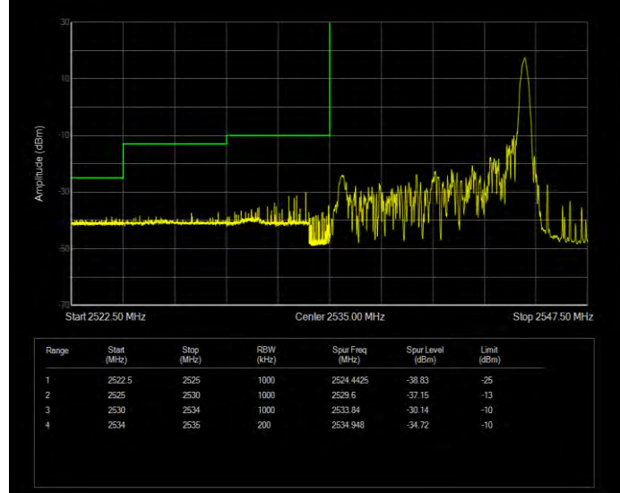
Band41(2535-2655) 16QAM BW=10MHz Channel=40090 RB Size=50 Position=#0 Extended
