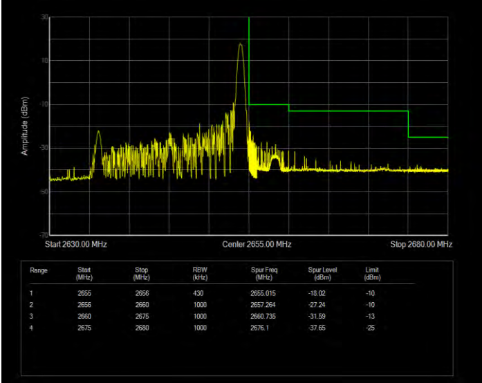
Band41(2535-2655) QPSK BW=20MHz Channel=41140 RB Size=100 Position=#0 Extended
