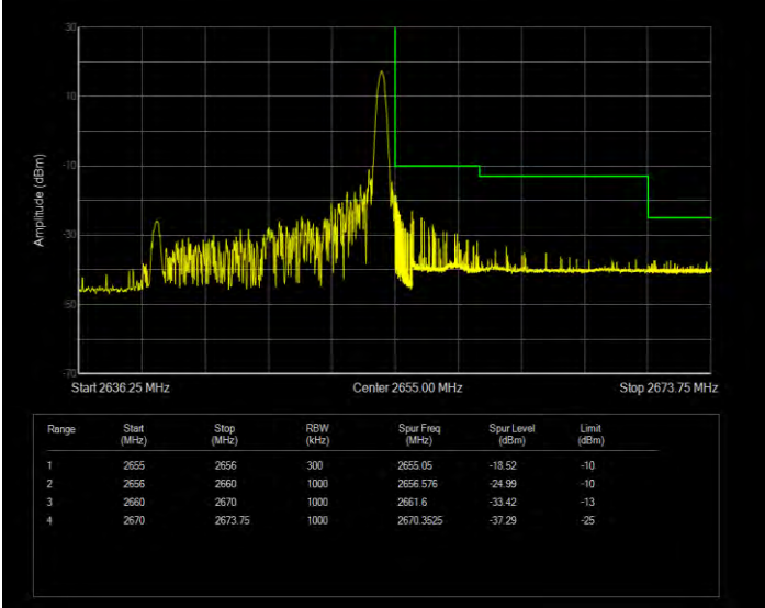
Band41(2535-2655) QPSK BW=15MHz Channel=41165 RB Size=75 Position=#0 Extended
