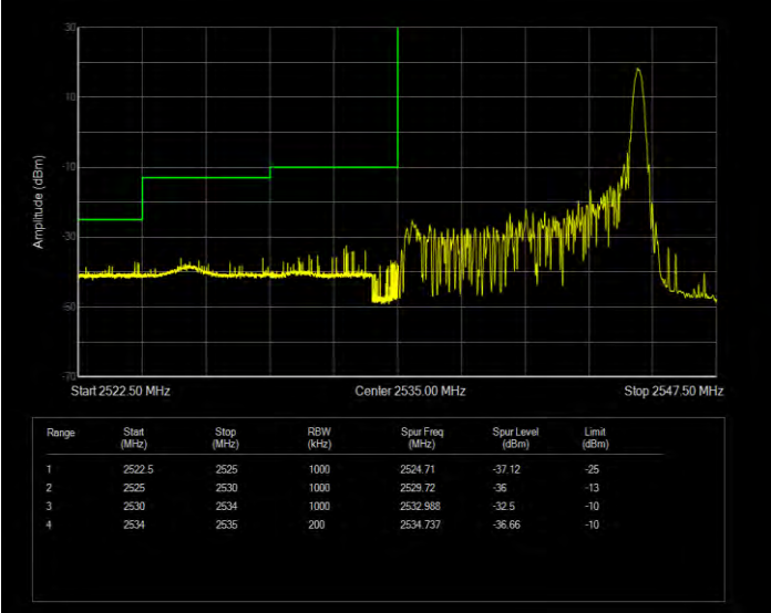
Band41(2535-2655) QPSK BW=10MHz Channel=40090 RB Size=50 Position=#0 Extended
