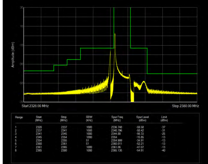
Band40(2350-2360) 16QAM BW=5MHz Channel=39225 RB Size=25 Position=#0 Extended
