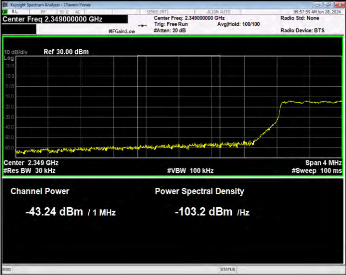
Band40(2350-2360) 16QAM BW=5MHz Channel=39175 RB Size=25 Position=#0 Normal
