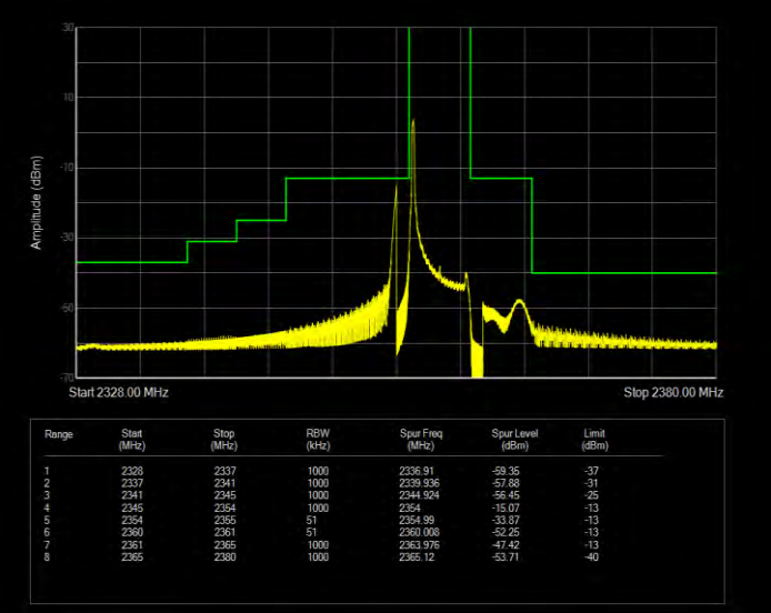
Band40(2350-2360) QPSK BW=5MHz Channel=39225 RB Size=25 Position=#0 Extended
