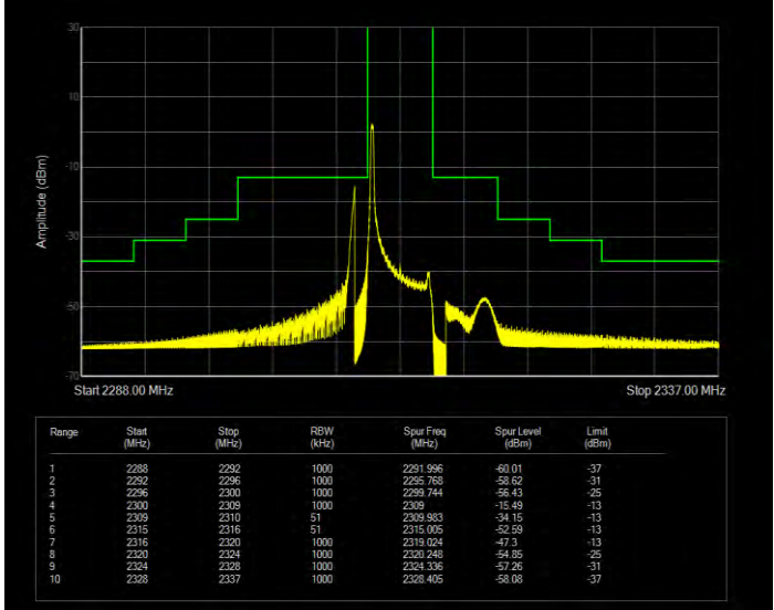
Band40(2305-2315) 16QAM BW=5MHz Channel=38775 RB Size=25 Position=#0 Extended
