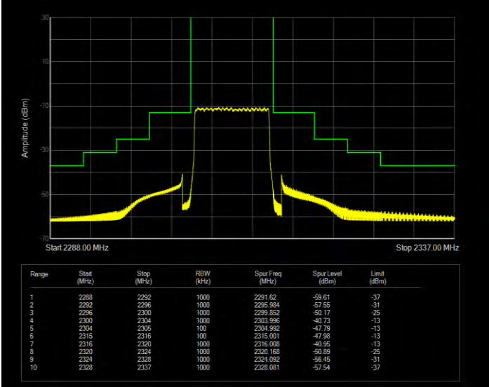
Band40(2305-2315) QPSK BW=5MHz Channel=38725 RB Size=1 Position=#0 Extended
