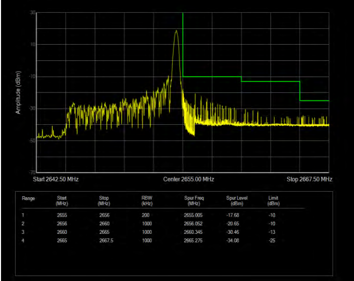
Band41(2535-2655) QPSK BW=10MHz Channel=41190 RB Size=50 Position=#0 Extended
