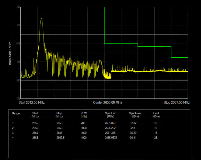
Band41(2535-2655) 16QAM BW=10MHz Channel=41190 RB Size=1 Position=#Max Extended
