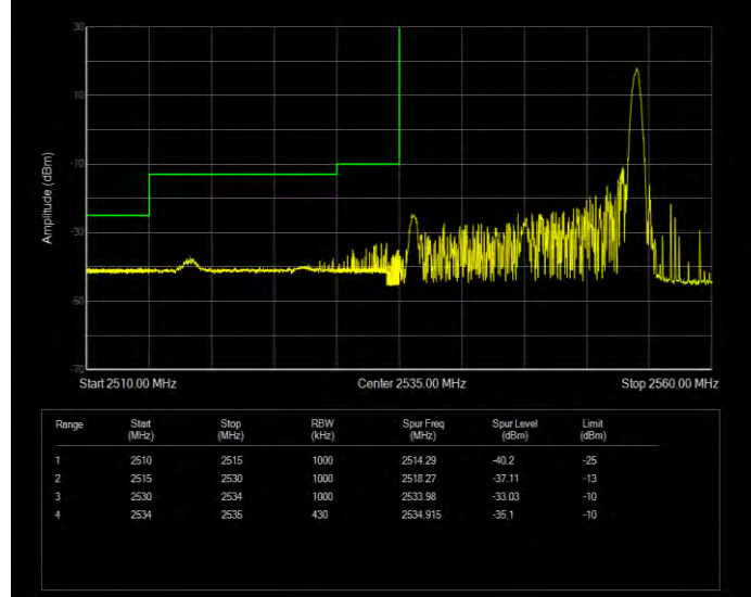
Band41(2535-2655) 16QAM BW=20MHz Channel=40140 RB Size=100 Position=#0 Extended
