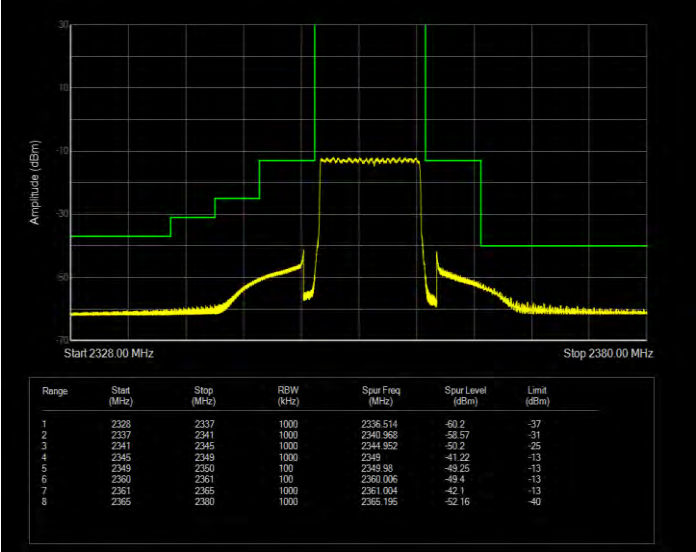
Band40(2350-2360) 16QAM BW=5MHz Channel=39175 RB Size=1 Position=#0 Extended
