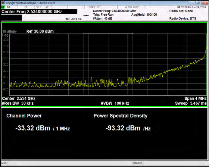
Band41(2535-2655) 16QAM BW=20MHz Channel=40140 RB Size=1 Position=#0 Normal
