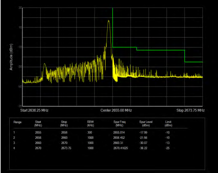
Band41(2535-2655) 16QAM BW=15MHz Channel=41165 RB Size=75 Position=#0 Extended
