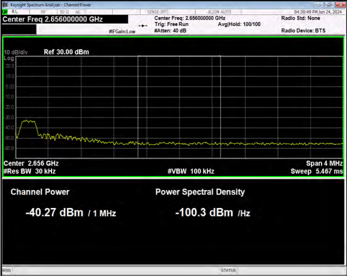
Band41(2535-2655) QPSK BW=15MHz Channel=41165 RB Size=1 Position=#0 Normal
