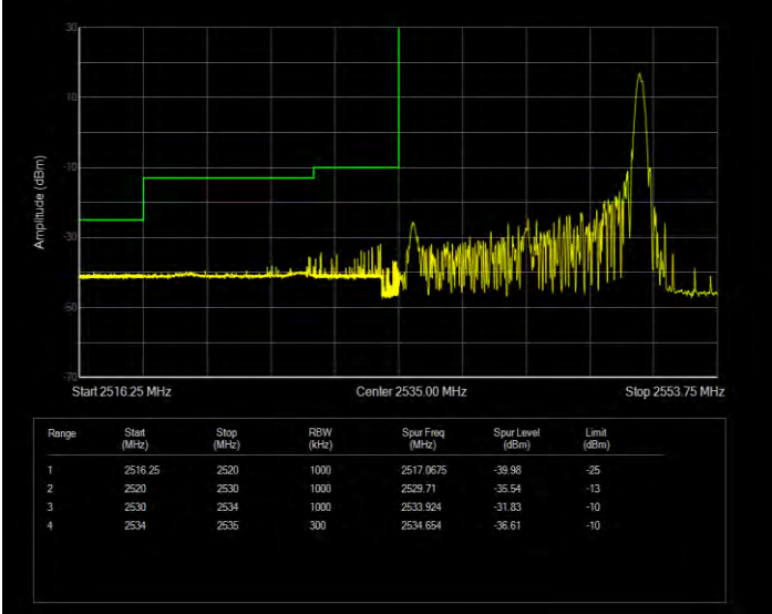
Band41(2535-2655) 16QAM BW=15MHz Channel=40115 RB Size=75 Position=#0 Extended
