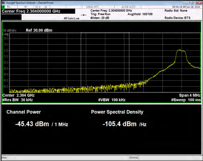
Band40(2305-2315) 16QAM BW=10MHz Channel=38750 RB Size=1 Position=#0 Normal
