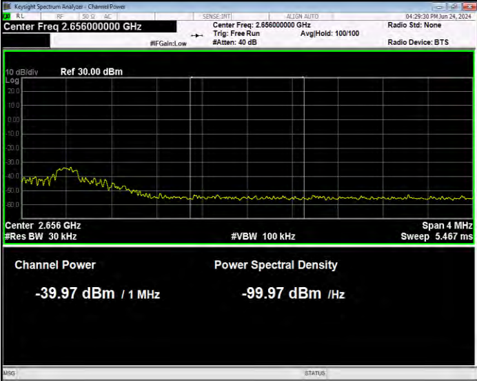
Band41(2535-2655) 16QAM BW=10MHz Channel=41190 RB Size=1 Position=#0 Normal
