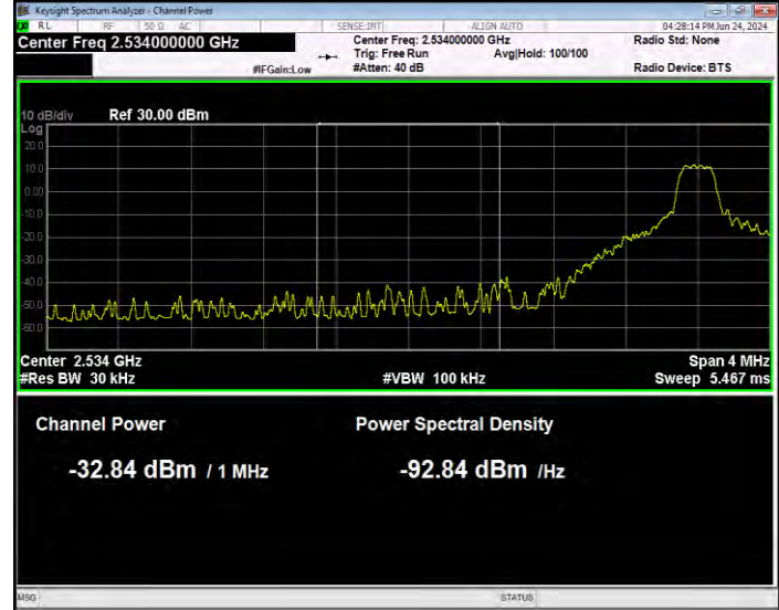
Band41(2535-2655) QPSK BW=10MHz Channel=40090 RB Size=1 Position=#0 Normal
