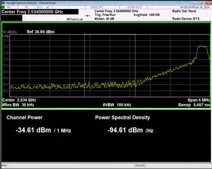
Band41(2535-2655) 16QAM BW=15MHz Channel=40115 RB Size=1 Position=#0 Normal
