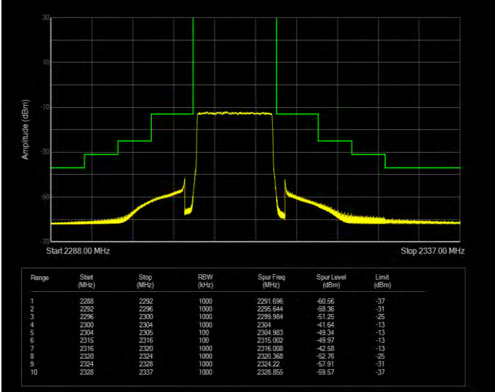
Band40(2305-2315) 16QAM BW=5MHz Channel=38725 RB Size=1 Position=#0 Extended
