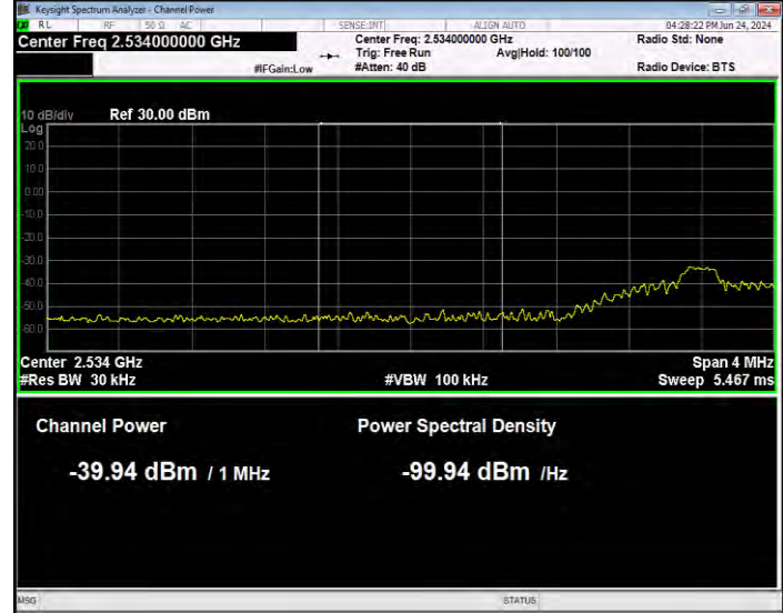
Band41(2535-2655) QPSK BW=10MHz Channel=40090 RB Size=1 Position=#Max Extended
