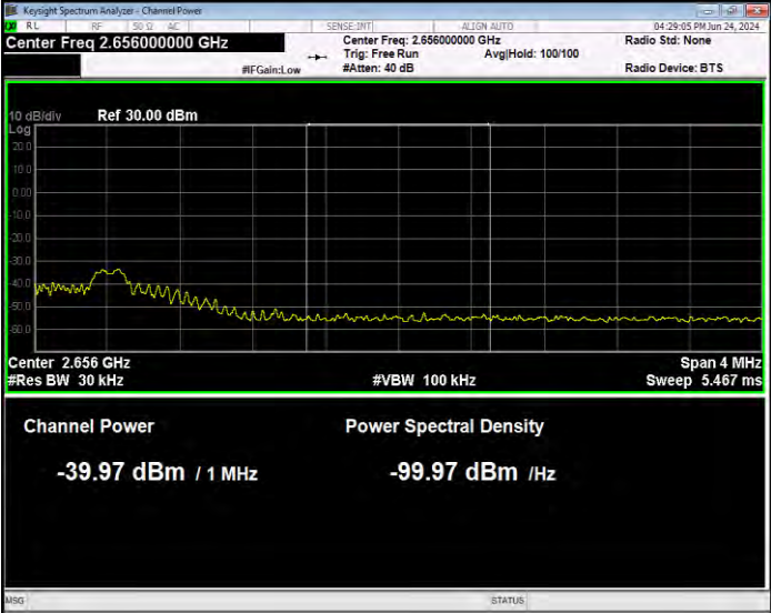
Band41(2535-2655) QPSK BW=10MHz Channel=41190 RB Size=1 Position=#0 Normal
