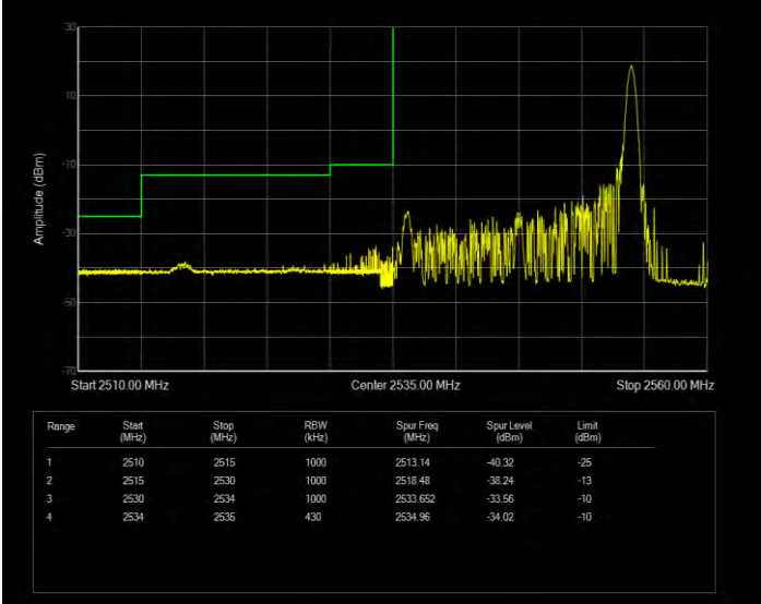
Band41(2535-2655) QPSK BW=20MHz Channel=40140 RB Size=100 Position=#0 Extended
