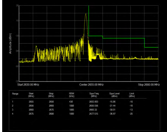
Band41(2535-2655) 16QAM BW=20MHz Channel=41140 RB Size=100 Position=#0 Extended
