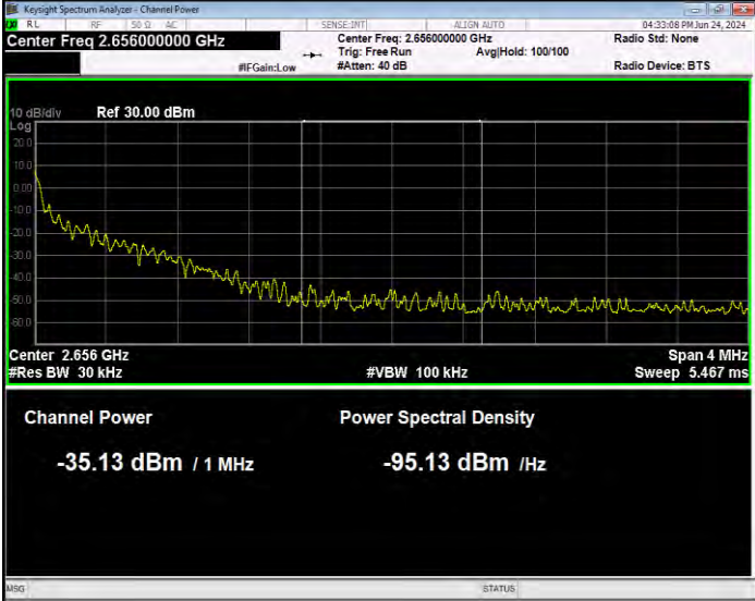
Band41(2535-2655) 16QAM BW=20MHz Channel=41140 RB Size=1 Position=#Max Extended
