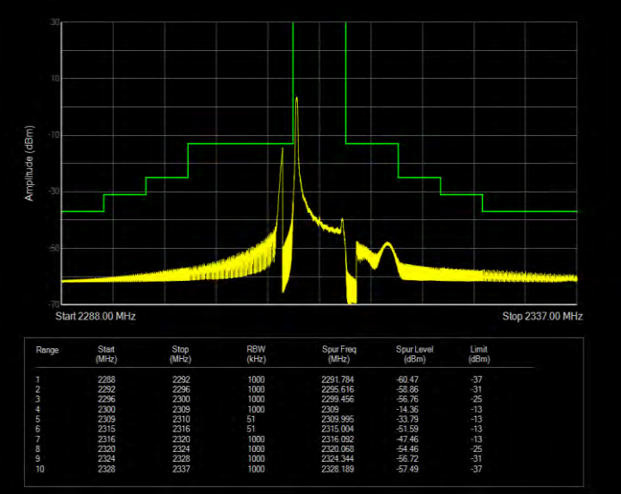
Band40(2305-2315) QPSK BW=5MHz Channel=38775 RB Size=25 Position=#0 Extended
