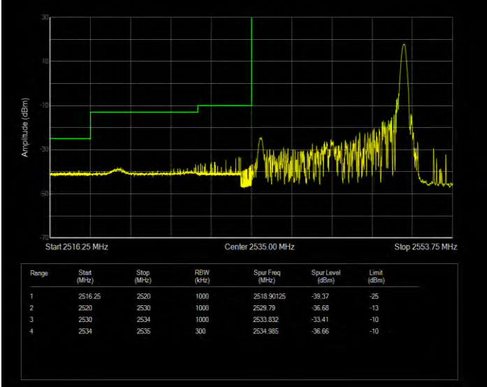
Band41(2535-2655) QPSK BW=15MHz Channel=40115 RB Size=75 Position=#0 Extended
