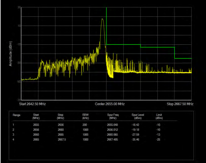
Band41(2535-2655) 16QAM BW=10MHz Channel=41190 RB Size=50 Position=#0 Extended
