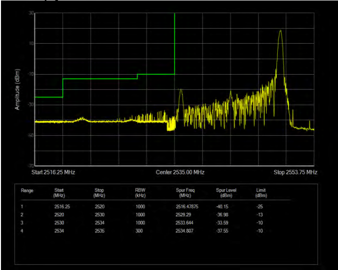
Band41(2535-2655) QPSK BW=15MHz Channel=40115 RB Size=75 Position=#0 Extended
