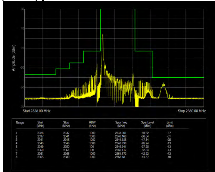
Band40(2350-2360) QPSK BW=10MHz Channel=39200 RB Size=50 Position=#0 Normal
