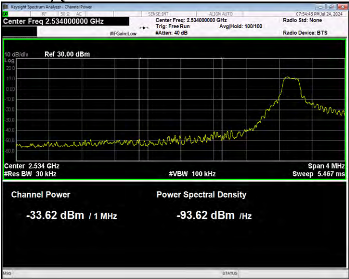
Band41(2535-2655) QPSK BW=5MHz Channel=40065 RB Size=1 Position=#0 Normal
