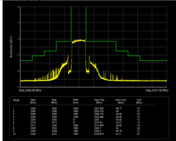
Band40(2305-2315) 16QAM BW=5MHz Channel=38775 RB Size=1 Position=#0 Normal
