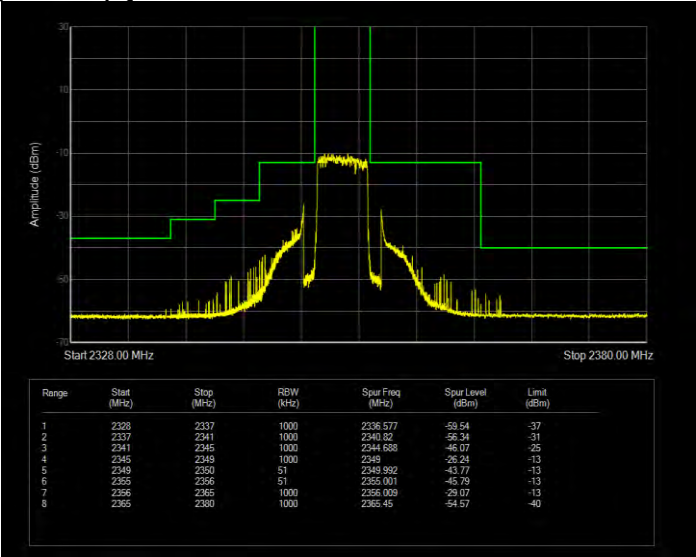
Band40(2350-2360) QPSK BW=5MHz Channel=39225 RB Size=1 Position=#0 Normal
