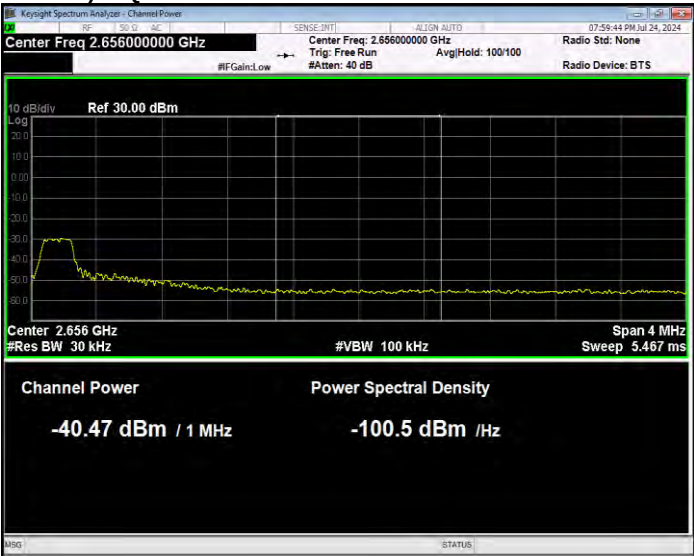
Band41(2535-2655) 16QAM BW=15MHz Channel=41165 RB Size=1 Position=#0 Normal
