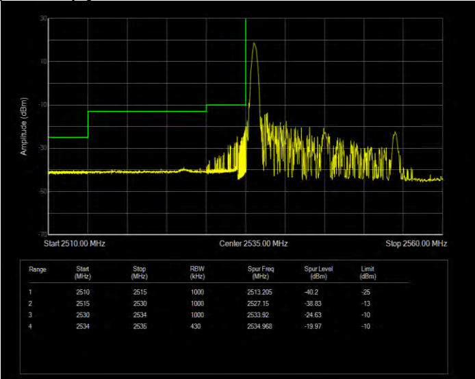
Band41(2535-2655) QPSK BW=20MHz Channel=40140 RB Size=1 Position=#Max Extended
