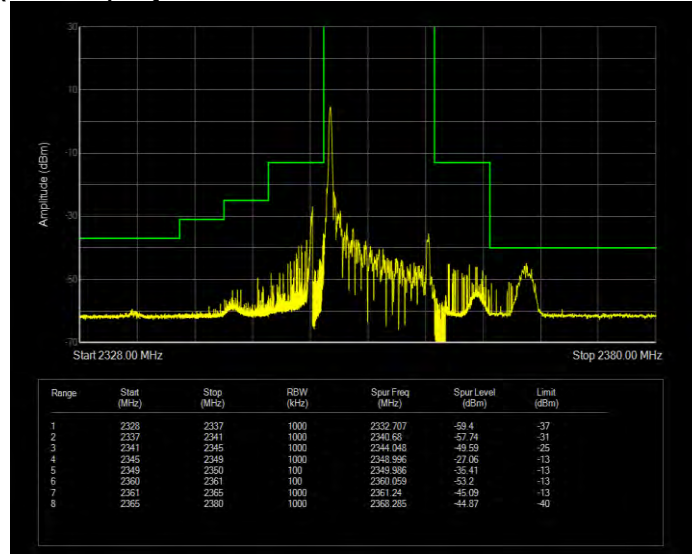
Band40(2350-2360) 16QAM BW=10MHz Channel=39200 RB Size=50 Position=#0 Normal
