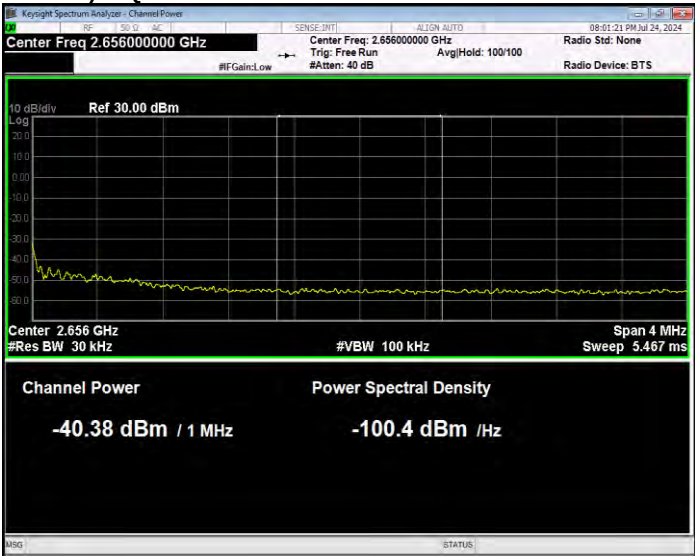
Band41(2535-2655) 16QAM BW=20MHz Channel=41140 RB Size=1 Position=#0 Normal
