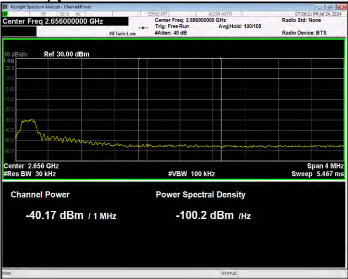
Band41(2535-2655) QPSK BW=15MHz Channel=41165 RB Size=1 Position=#0 Normal
