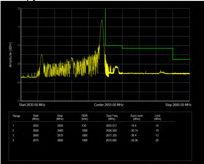
Band41(2535-2655) QPSK BW=20MHz Channel=41140 RB Size=100 Position=#0 Extended
