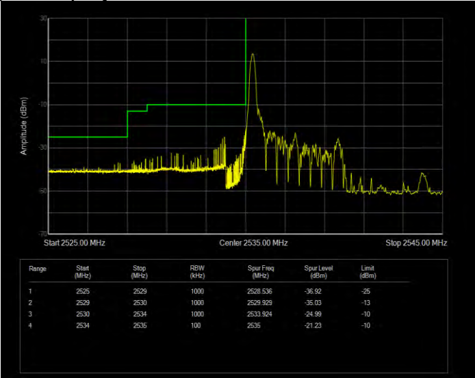
Band41(2535-2655) 16QAM BW=5MHz Channel=40065 RB Size=1 Position=#Max Extended
