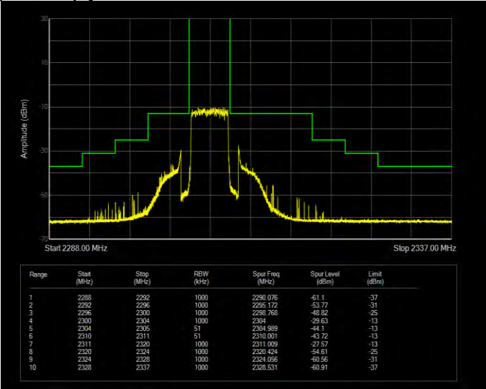
Band40(2305-2315) QPSK BW=5MHz Channel=38775 RB Size=1 Position=#0 Normal
