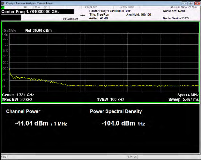
Band66 16QAM BW=20MHz Channel=132572 RB Size=1 Position=#0 Normal
