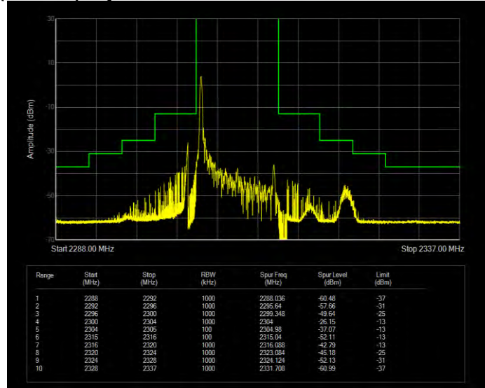
Band40(2305-2315) 16QAM BW=10MHz Channel=38750 RB Size=50 Position=#0 Normal
