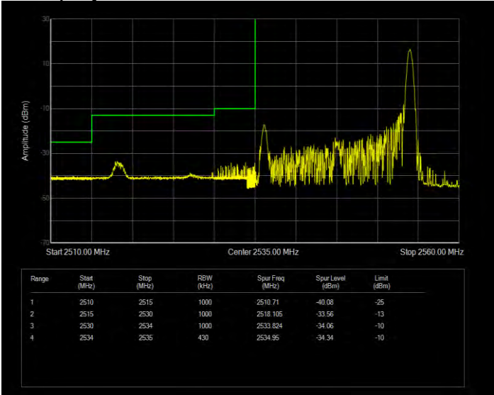
Band41(2535-2655) 16QAM BW=20MHz Channel=40140 RB Size=100 Position=#0 Extended
