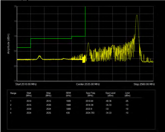
Band41(2535-2655) QPSK BW=20MHz Channel=40140 RB Size=100 Position=#0 Extended
