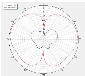
Phi=0 freq=2400MHz
