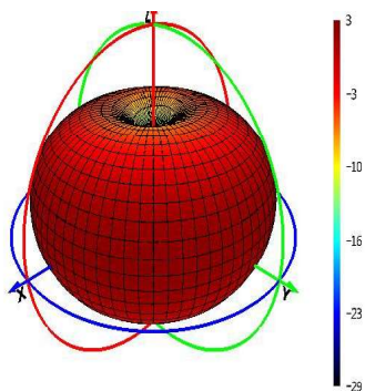
Phi=90 freq=5300MHz
