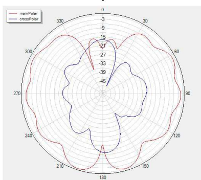
Phi=90 freq=5300MHz
