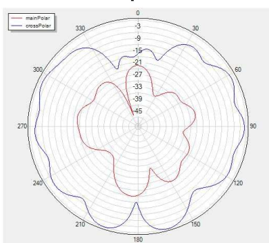
Phi=0 freq=5300MHz
