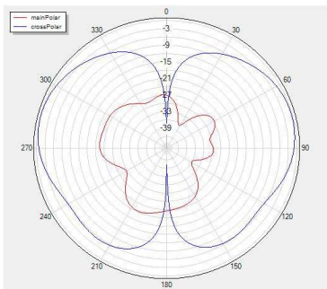
Phi=90 freq=2400MHz
