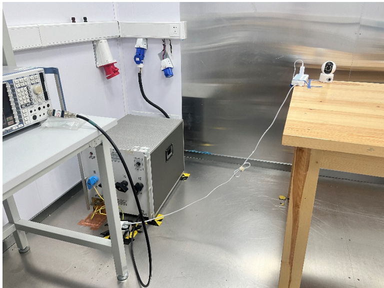
Conducted Emission
