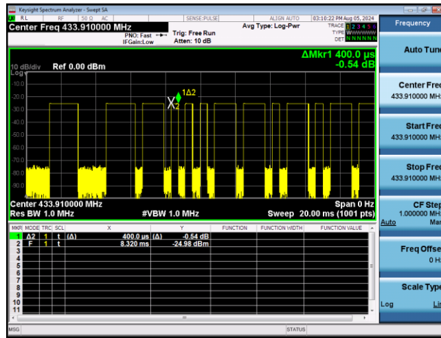
(Time per burst: 0.40 ms*8pcs)
