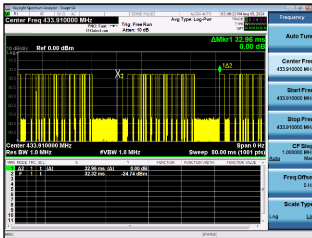
(Transmit cycle 32.96ms)
