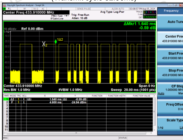
(Time per burst: 1.64ms*2pcs)
